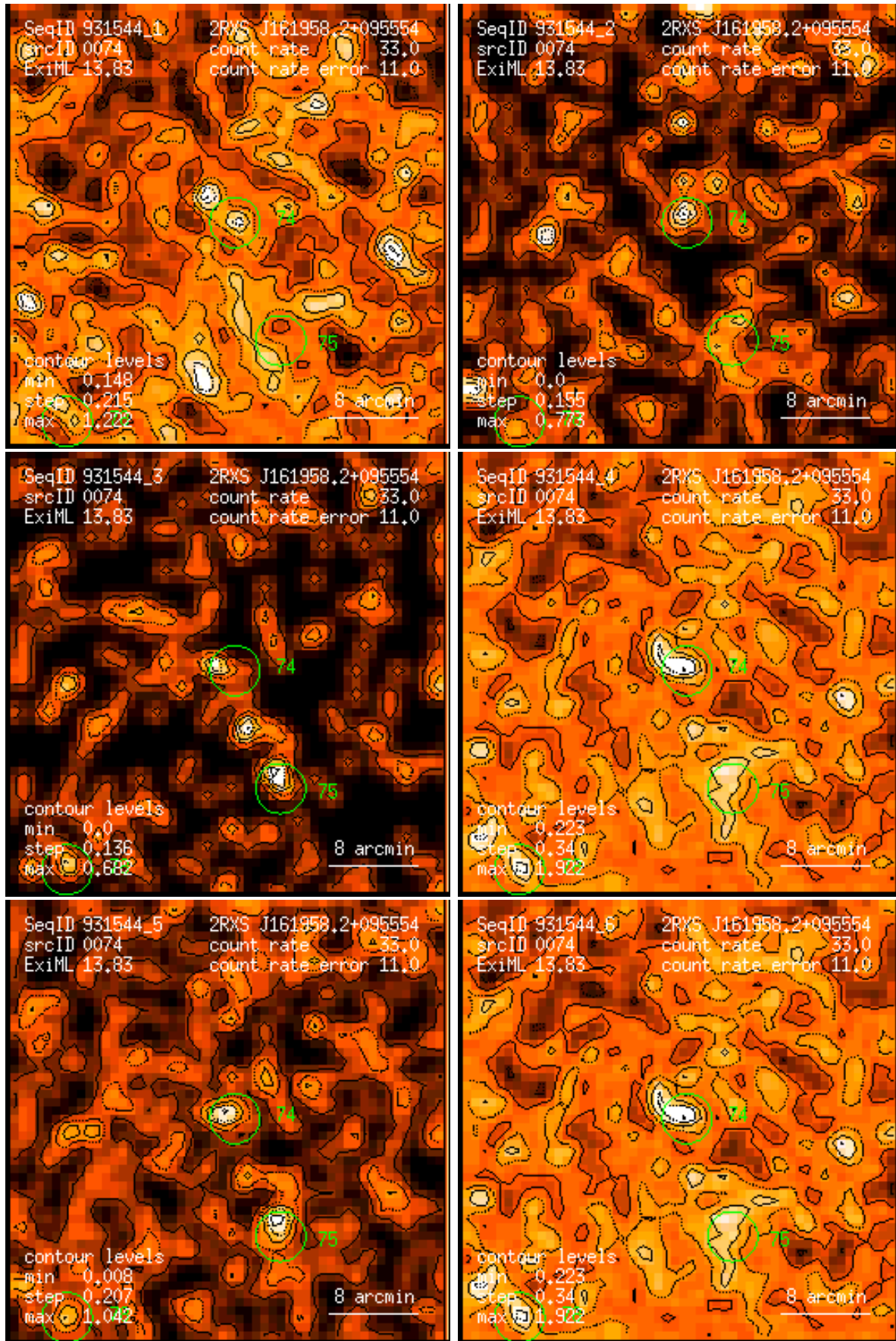
Figure 74: RASS 931544: detection 0074: band rate images, Gaussian filter: (1) PSPC channels 11 – 41, (2) 52 – 90, (3) 91 – 201, (4) 11 – 235, (5) 52 – 201, (6) 11 – 201. Broad band rates in counts/ks. Band rate contour levels in counts/ks/arcmin 2 .
