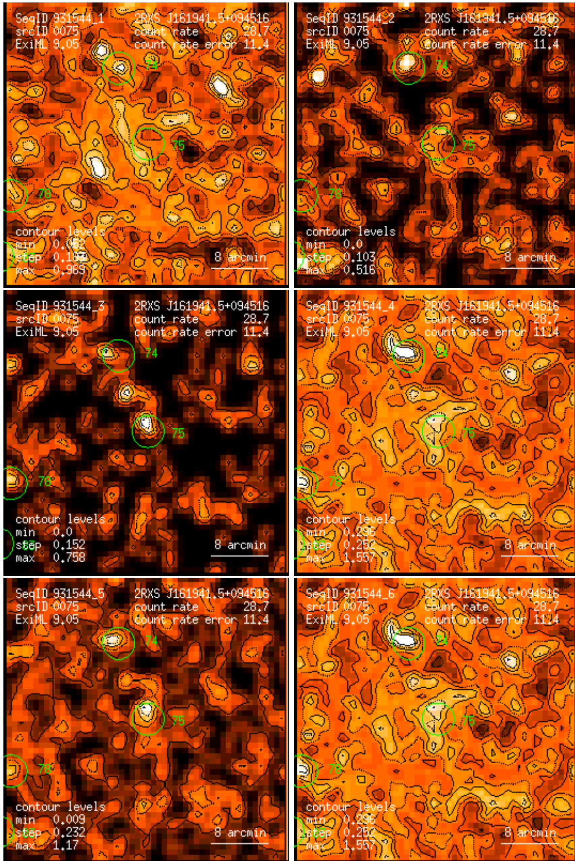
Figure 75: RASS 931544: detection 0075: band rate images, Gaussian filter: (1) PSPC channels 11 – 41, (2) 52 – 90, (3) 91 – 201, (4) 11 – 235, (5) 52 – 201, (6) 11 – 201. Broad band rates in counts/ks. Band rate contour levels in counts/ks/arcmin 2 .
