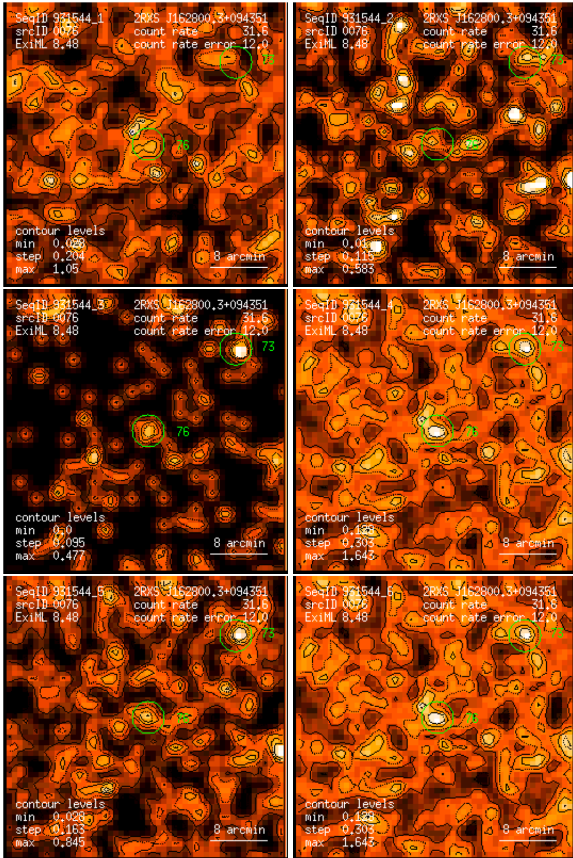
Figure 76: RASS 931544: detection 0076: band rate images, Gaussian filter: (1) PSPC channels 11 – 41, (2) 52 – 90, (3) 91 – 201, (4) 11 – 235, (5) 52 – 201, (6) 11 – 201. Broad band rates in counts/ks. Band rate contour levels in counts/ks/arcmin 2 .
