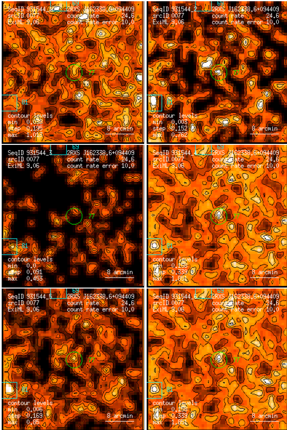
Figure 77: RASS 931544: detection 0077: band rate images, Gaussian filter: (1) PSPC channels 11 – 41, (2) 52 – 90, (3) 91 – 201, (4) 11 – 235, (5) 52 – 201, (6) 11 – 201. Broad band rates in counts/ks. Band rate contour levels in counts/ks/arcmin 2 .
