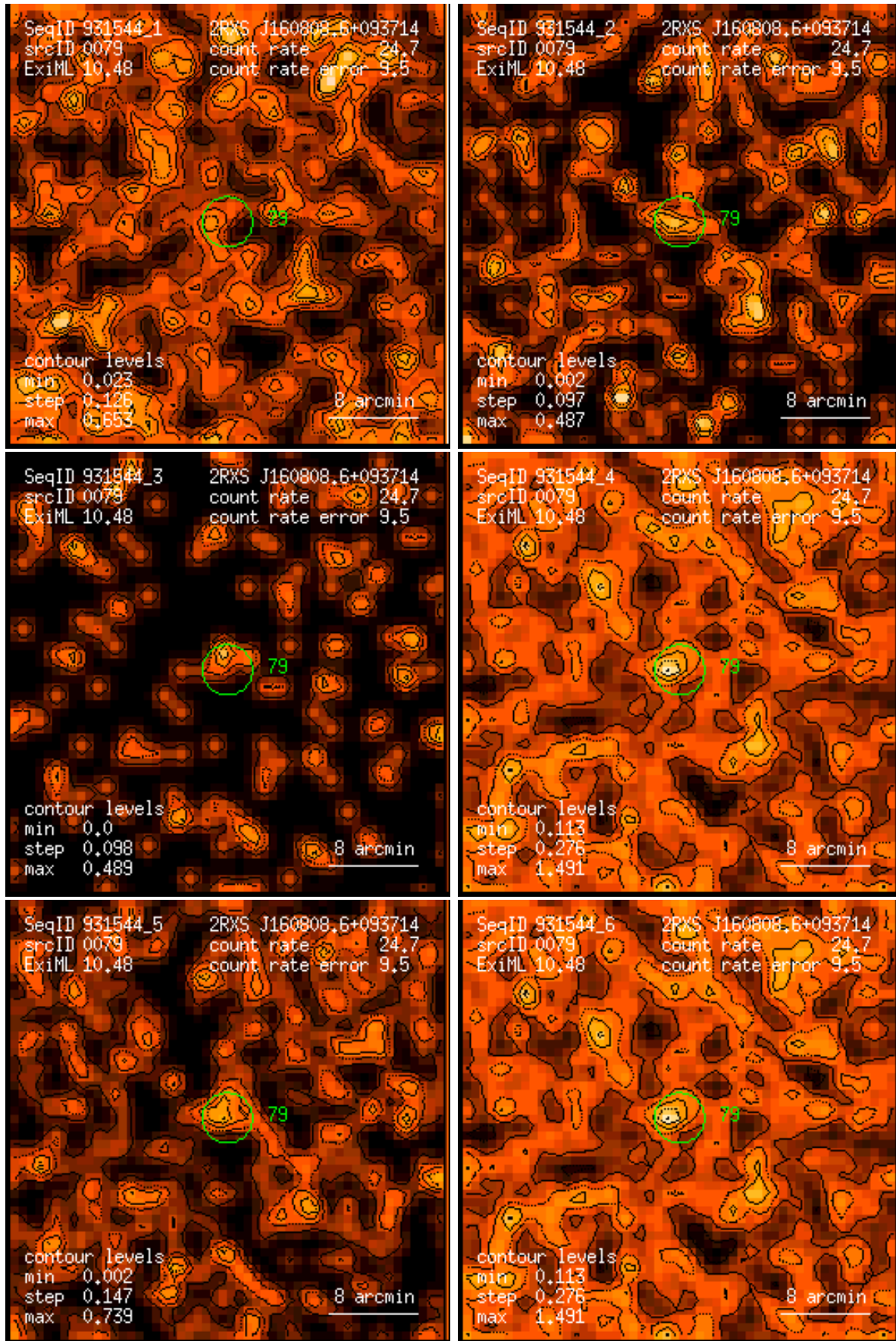
Figure 79: RASS 931544: detection 0079: band rate images, Gaussian filter: (1) PSPC channels 11 – 41, (2) 52 – 90, (3) 91 – 201, (4) 11 – 235, (5) 52 – 201, (6) 11 – 201. Broad band rates in counts/ks. Band rate contour levels in counts/ks/arcmin 2 .
