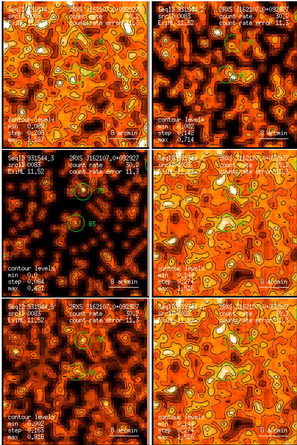
Figure 83: RASS 931544: detection 0083: band rate images, Gaussian filter: (1) PSPC channels 11 – 41, (2) 52 – 90, (3) 91 – 201, (4) 11 – 235, (5) 52 – 201, (6) 11 – 201. Broad band rates in counts/ks. Band rate contour levels in counts/ks/arcmin 2 .
