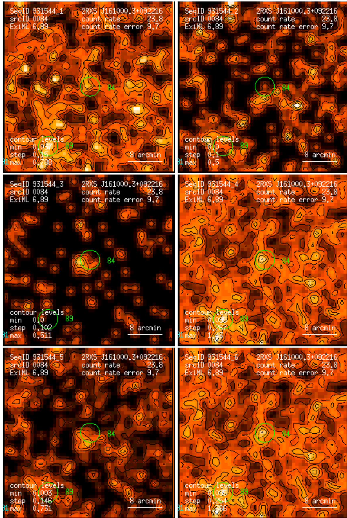
Figure 84: RASS 931544: detection 0084: band rate images, Gaussian filter: (1) PSPC channels 11 – 41, (2) 52 – 90, (3) 91 – 201, (4) 11 – 235, (5) 52 – 201, (6) 11 – 201. Broad band rates in counts/ks. Band rate contour levels in counts/ks/arcmin 2 .
