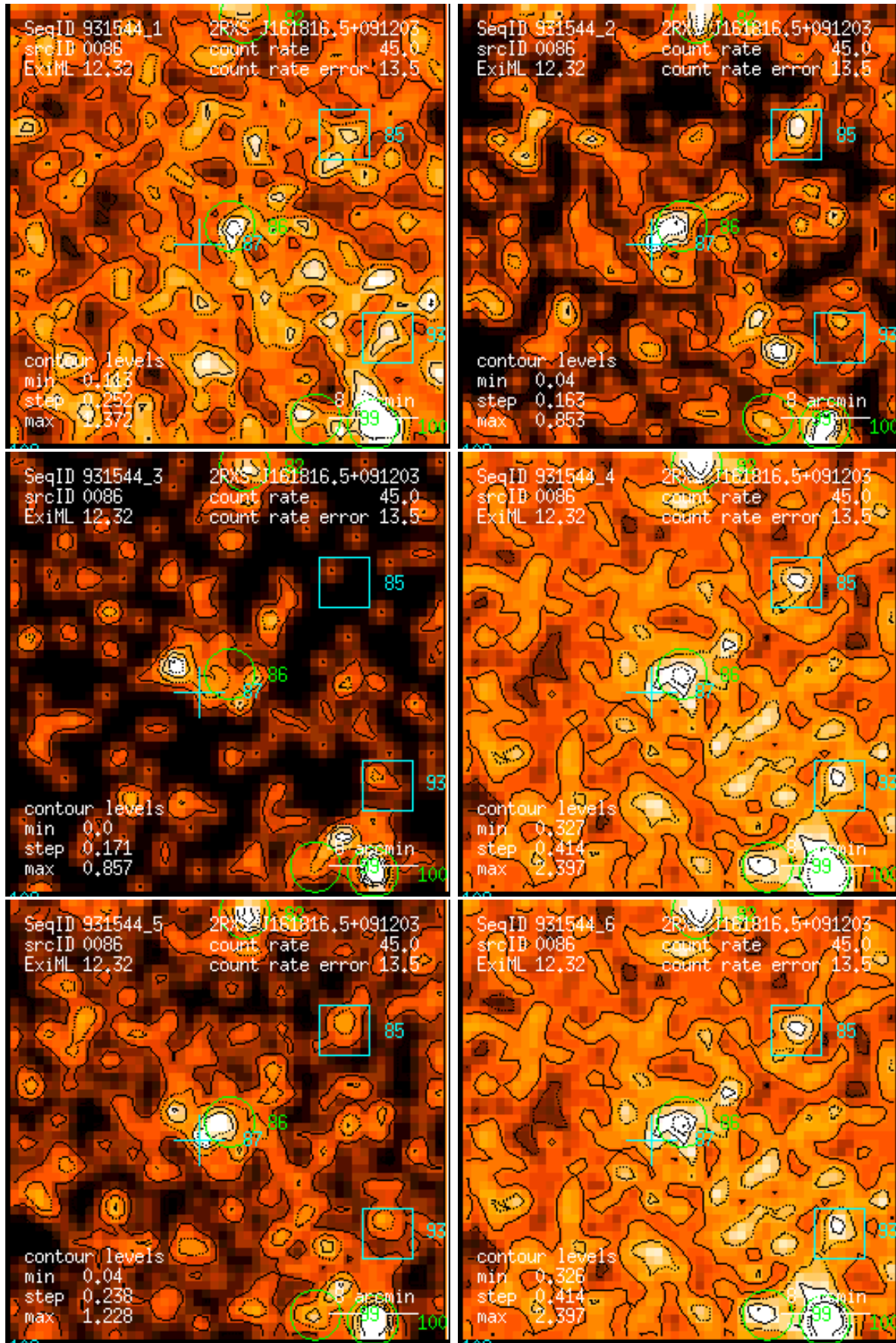
Figure 86: RASS 931544: detection 0086: band rate images, Gaussian filter: (1) PSPC channels 11 – 41, (2) 52 – 90, (3) 91 – 201, (4) 11 – 235, (5) 52 – 201, (6) 11 – 201. Broad band rates in counts/ks. Band rate contour levels in counts/ks/arcmin 2 .
