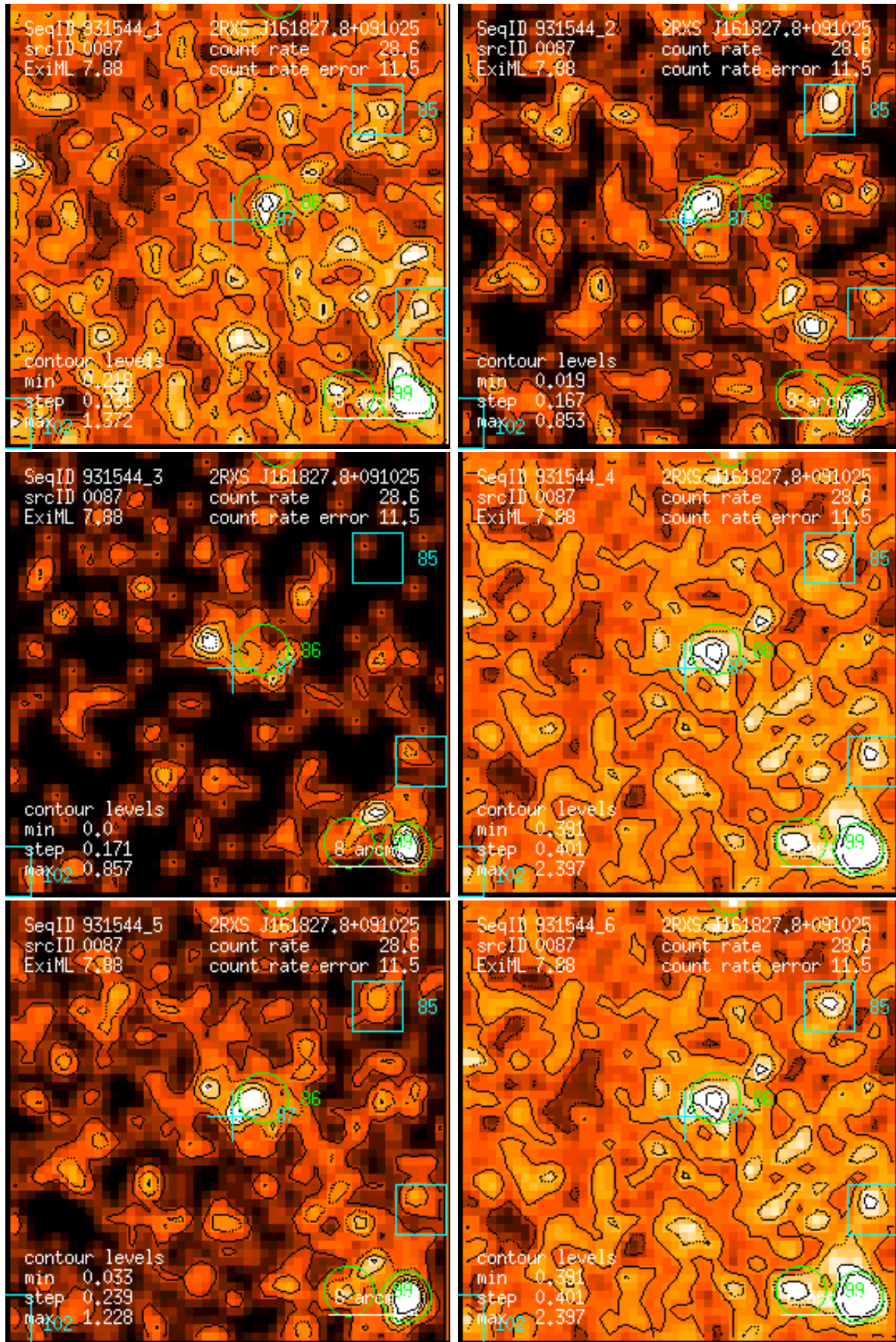
Figure 87: RASS 931544: detection 0087: band rate images, Gaussian filter: (1) PSPC channels 11 – 41, (2) 52 – 90, (3) 91 – 201, (4) 11 – 235, (5) 52 – 201, (6) 11 – 201. Broad band rates in counts/ks. Band rate contour levels in counts/ks/arcmin 2 .
