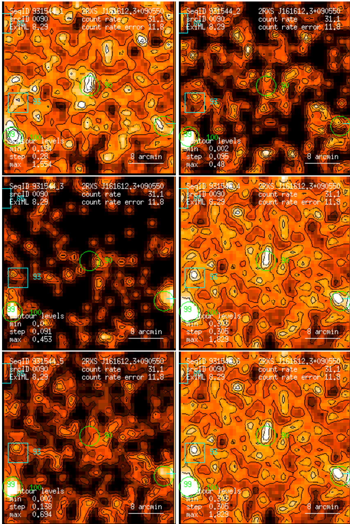
Figure 90: RASS 931544: detection 0090: band rate images, Gaussian filter: (1) PSPC channels 11 – 41, (2) 52 – 90, (3) 91 – 201, (4) 11 – 235, (5) 52 – 201, (6) 11 – 201. Broad band rates in counts/ks. Band rate contour levels in counts/ks/arcmin 2 .
