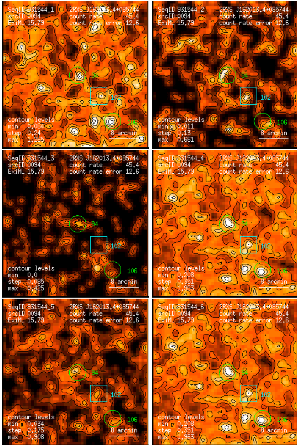
Figure 94: RASS 931544: detection 0094: band rate images, Gaussian filter: (1) PSPC channels 11 – 41, (2) 52 – 90, (3) 91 – 201, (4) 11 – 235, (5) 52 – 201, (6) 11 – 201. Broad band rates in counts/ks. Band rate contour levels in counts/ks/arcmin 2 .
