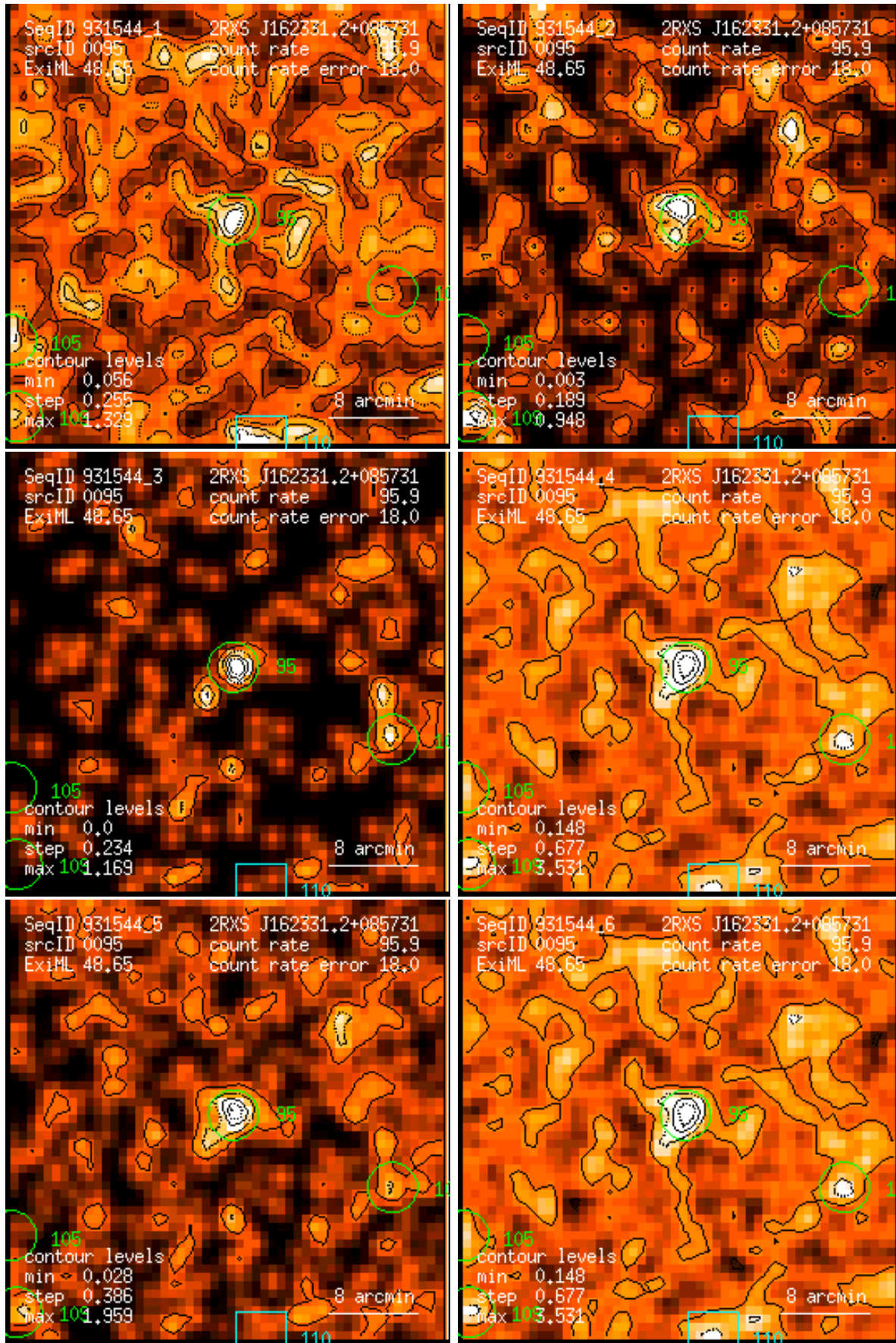
Figure 95: RASS 931544: detection 0095: band rate images, Gaussian filter: (1) PSPC channels 11 – 41, (2) 52 – 90, (3) 91 – 201, (4) 11 – 235, (5) 52 – 201, (6) 11 – 201. Broad band rates in counts/ks. Band rate contour levels in counts/ks/arcmin 2 .
