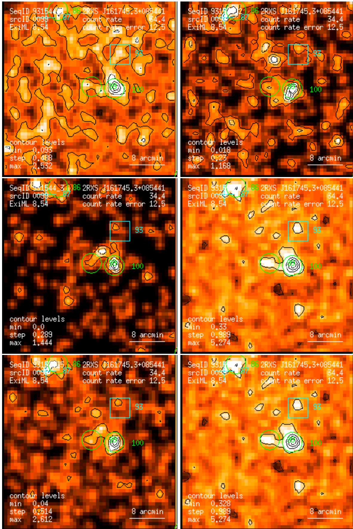
Figure 99: RASS 931544: detection 0099: band rate images, Gaussian filter: (1) PSPC channels 11 – 41, (2) 52 – 90, (3) 91 – 201, (4) 11 – 235, (5) 52 – 201, (6) 11 – 201. Broad band rates in counts/ks. Band rate contour levels in counts/ks/arcmin 2 .
