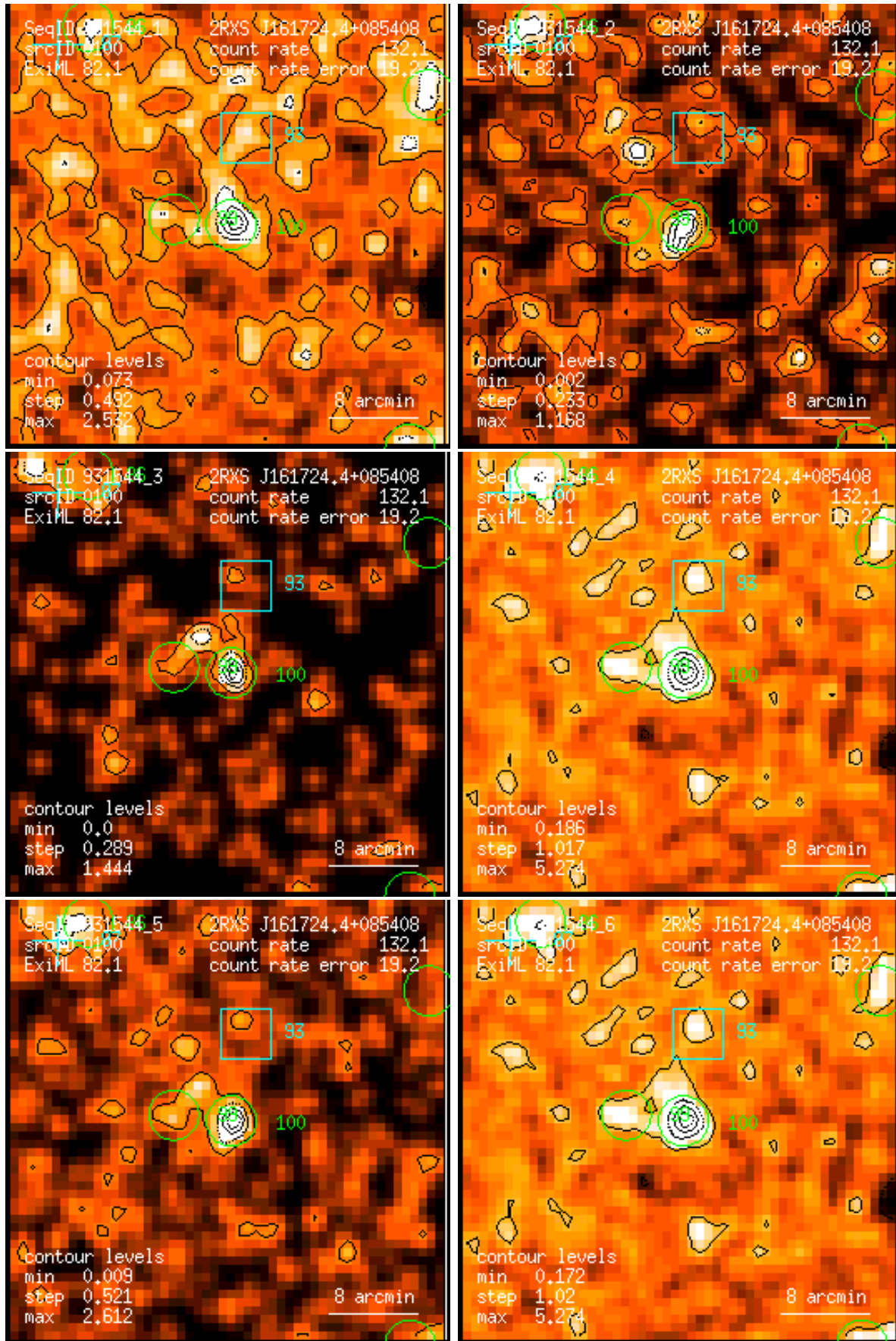
Figure 100: RASS 931544: detection 0100: band rate images, Gaussian filter: (1) PSPC channels 11 – 41, (2) 52 – 90, (3) 91 – 201, (4) 11 – 235, (5) 52 – 201, (6) 11 – 201. Broad band rates in counts/ks. Band rate contour levels in counts/ks/arcmin 2 .
