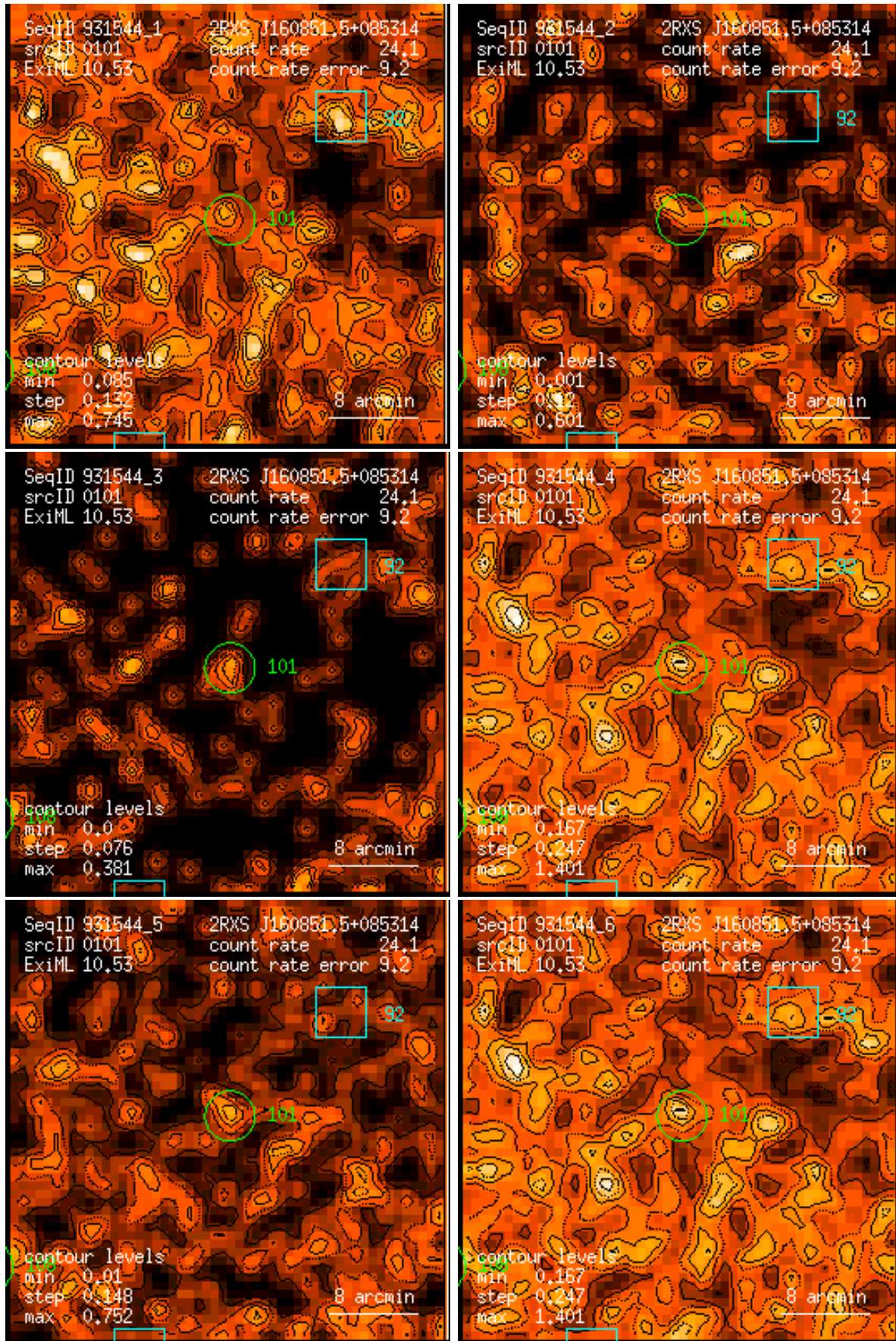
Figure 101: RASS 931544: detection 0101: band rate images, Gaussian filter: (1) PSPC channels 11 – 41, (2) 52 – 90, (3) 91 – 201, (4) 11 – 235, (5) 52 – 201, (6) 11 – 201. Broad band rates in counts/ks. Band rate contour levels in counts/ks/arcmin 2 .
