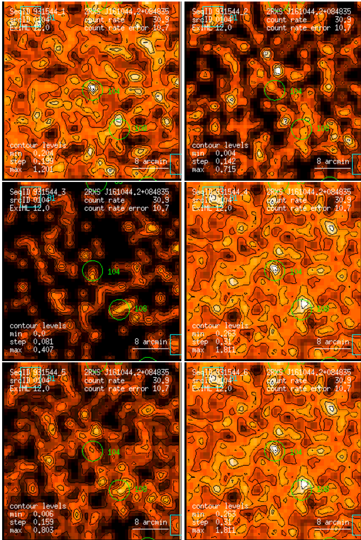
Figure 104: RASS 931544: detection 0104: band rate images, Gaussian filter: (1) PSPC channels 11 – 41, (2) 52 – 90, (3) 91 – 201, (4) 11 – 235, (5) 52 – 201, (6) 11 – 201. Broad band rates in counts/ks. Band rate contour levels in counts/ks/arcmin 2 .
