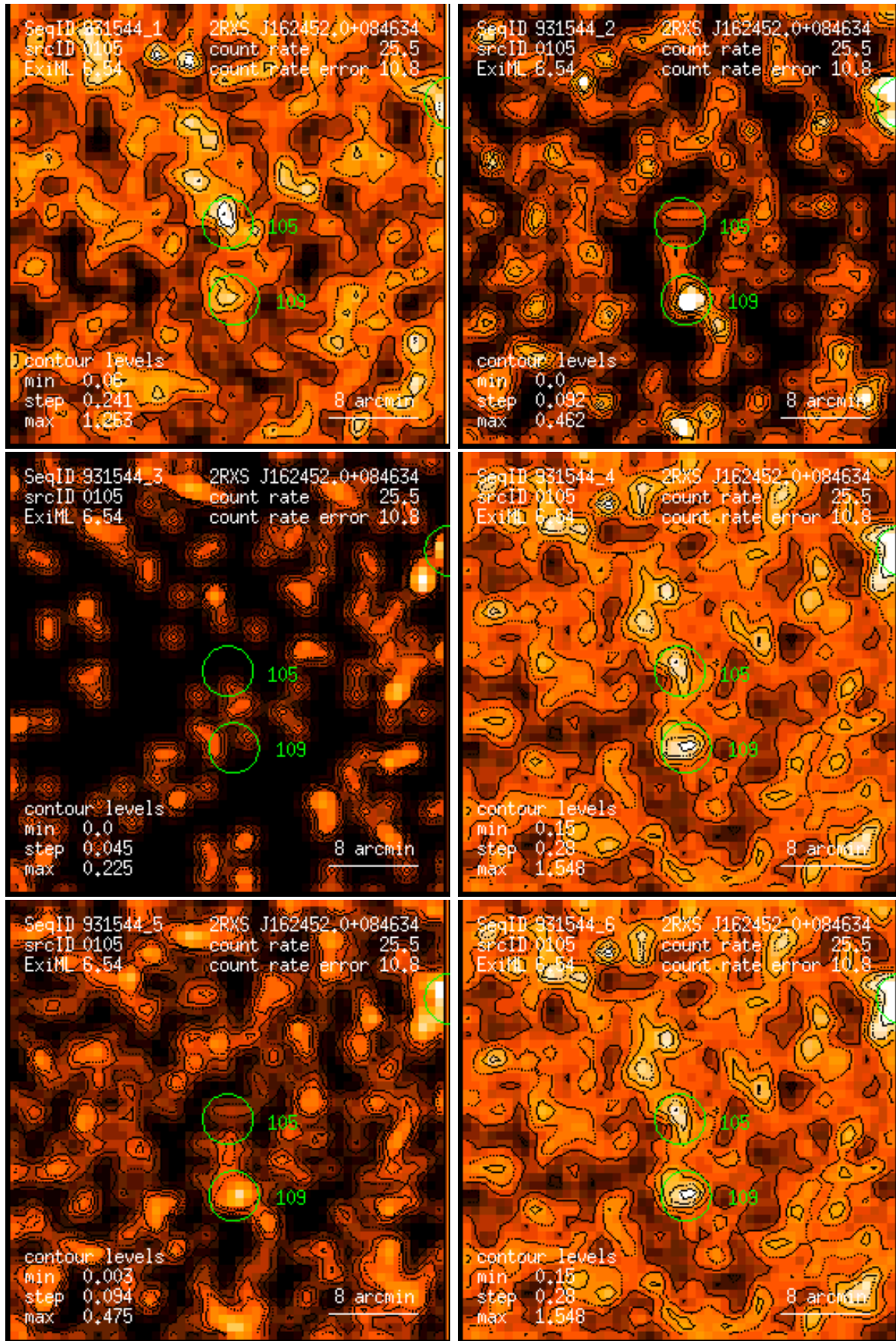
Figure 105: RASS 931544: detection 0105: band rate images, Gaussian filter: (1) PSPC channels 11 – 41, (2) 52 – 90, (3) 91 – 201, (4) 11 – 235, (5) 52 – 201, (6) 11 – 201. Broad band rates in counts/ks. Band rate contour levels in counts/ks/arcmin 2 .
