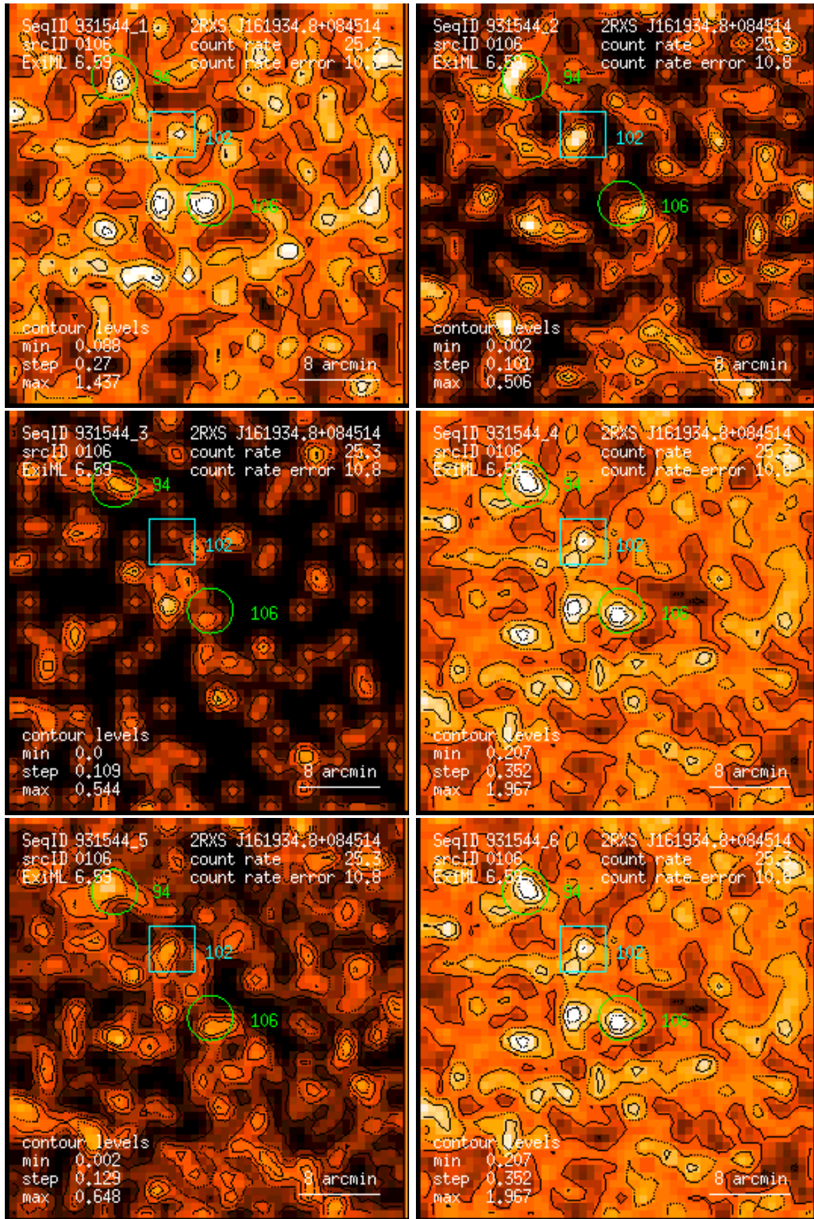
Figure 106: RASS 931544: detection 0106: band rate images, Gaussian filter: (1) PSPC channels 11 – 41, (2) 52 – 90, (3) 91 – 201, (4) 11 – 235, (5) 52 – 201, (6) 11 – 201. Broad band rates in counts/ks. Band rate contour levels in counts/ks/arcmin 2 .
