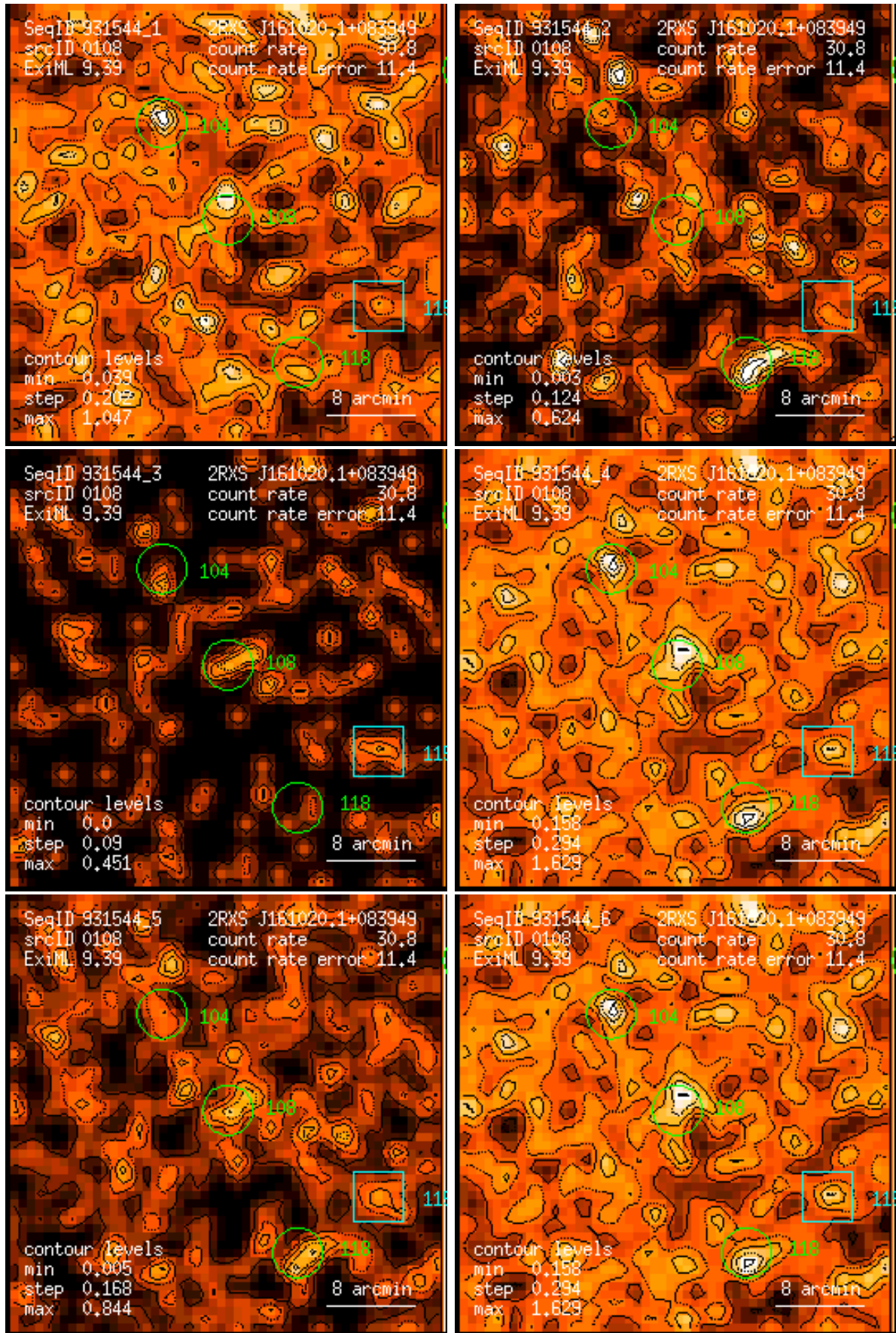
Figure 108: RASS 931544: detection 0108: band rate images, Gaussian filter: (1) PSPC channels 11 – 41, (2) 52 – 90, (3) 91 – 201, (4) 11 – 235, (5) 52 – 201, (6) 11 – 201. Broad band rates in counts/ks. Band rate contour levels in counts/ks/arcmin 2 .
