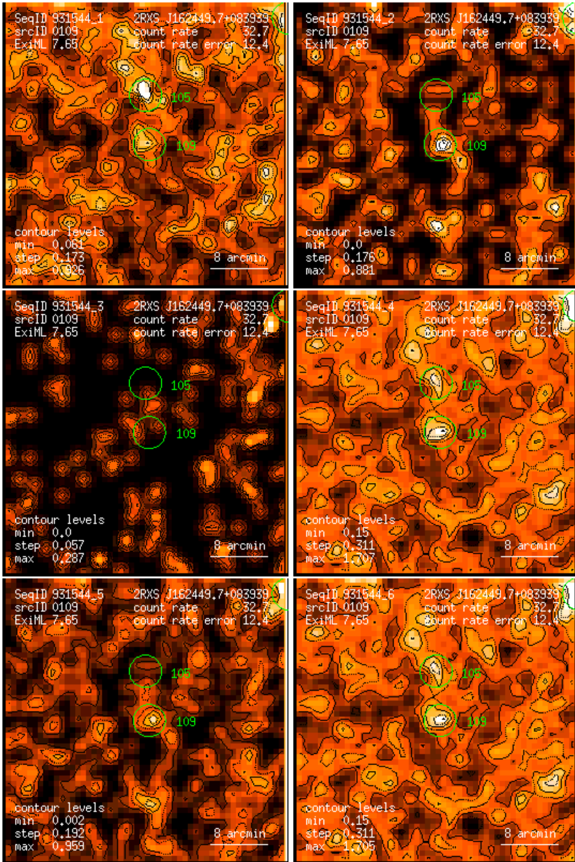
Figure 109: RASS 931544: detection 0109: band rate images, Gaussian filter: (1) PSPC channels 11 – 41, (2) 52 – 90, (3) 91 – 201, (4) 11 – 235, (5) 52 – 201, (6) 11 – 201. Broad band rates in counts/ks. Band rate contour levels in counts/ks/arcmin 2 .
