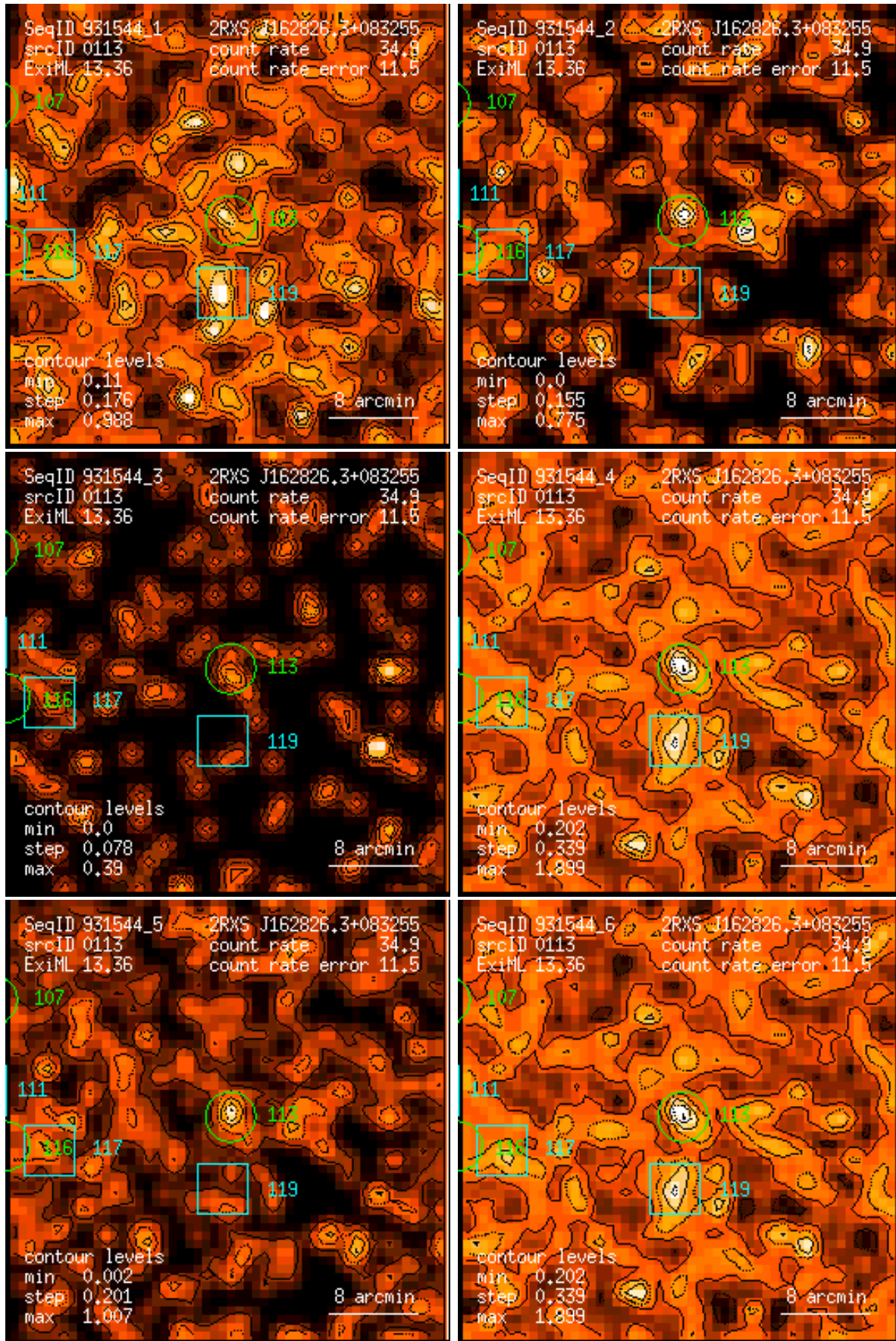
Figure 113: RASS 931544: detection 0113: band rate images, Gaussian filter: (1) PSPC channels 11 – 41, (2) 52 – 90, (3) 91 – 201, (4) 11 – 235, (5) 52 – 201, (6) 11 – 201. Broad band rates in counts/ks. Band rate contour levels in counts/ks/arcmin 2 .
