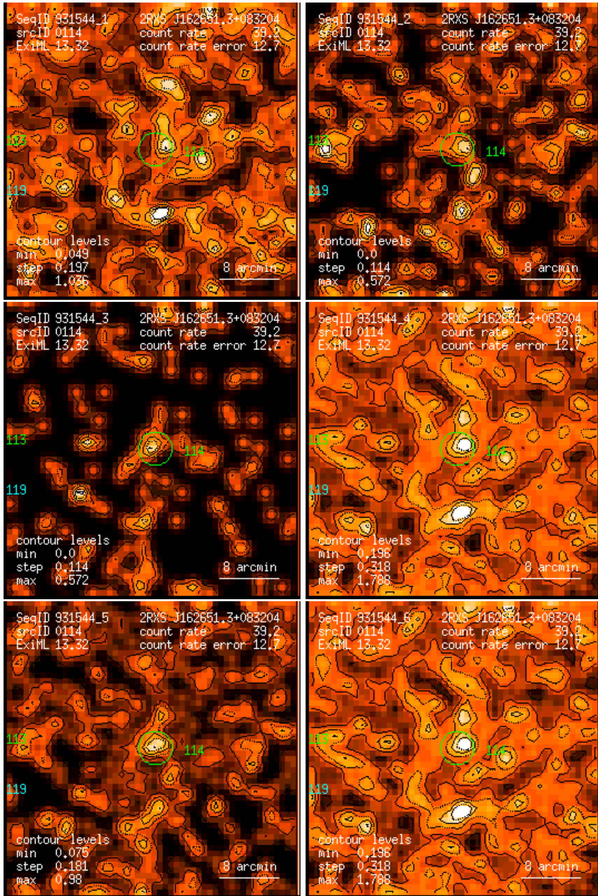
Figure 114: RASS 931544: detection 0114: band rate images, Gaussian filter: (1) PSPC channels 11 – 41, (2) 52 – 90, (3) 91 – 201, (4) 11 – 235, (5) 52 – 201, (6) 11 – 201. Broad band rates in counts/ks. Band rate contour levels in counts/ks/arcmin 2 .
