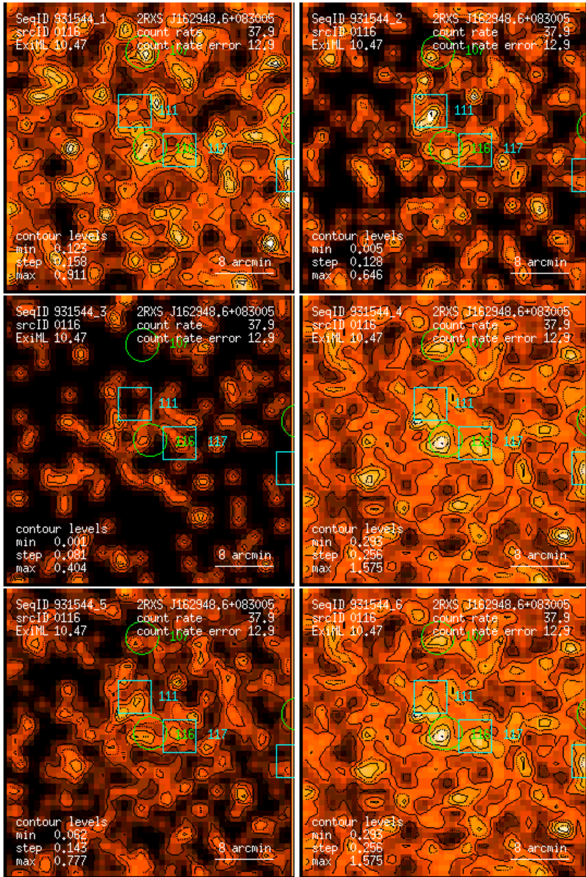
Figure 116: RASS 931544: detection 0116: band rate images, Gaussian filter: (1) PSPC channels 11 – 41, (2) 52 – 90, (3) 91 – 201, (4) 11 – 235, (5) 52 – 201, (6) 11 – 201. Broad band rates in counts/ks. Band rate contour levels in counts/ks/arcmin 2 .
