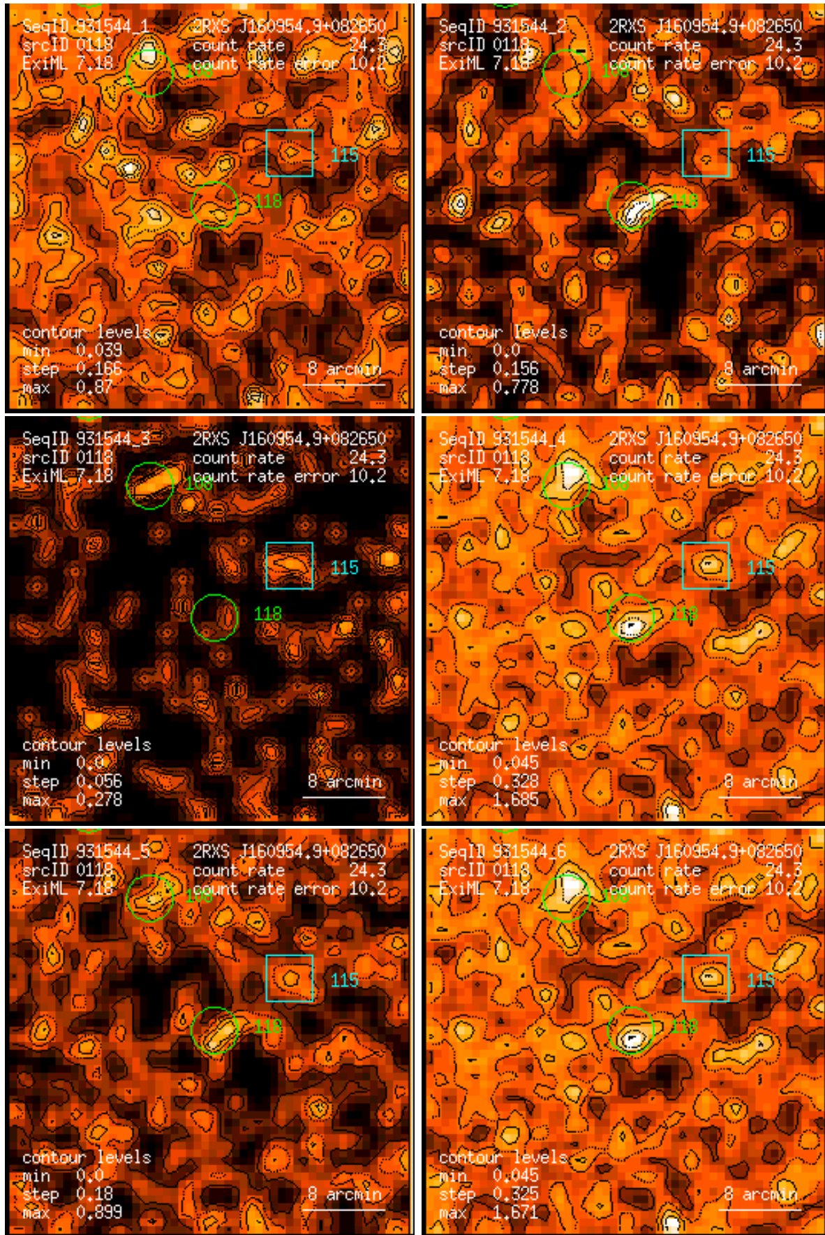
Figure 118: RASS 931544: detection 0118: band rate images, Gaussian filter: (1) PSPC channels 11 – 41, (2) 52 – 90, (3) 91 – 201, (4) 11 – 235, (5) 52 – 201, (6) 11 – 201. Broad band rates in counts/ks. Band rate contour levels in counts/ks/arcmin 2 .
