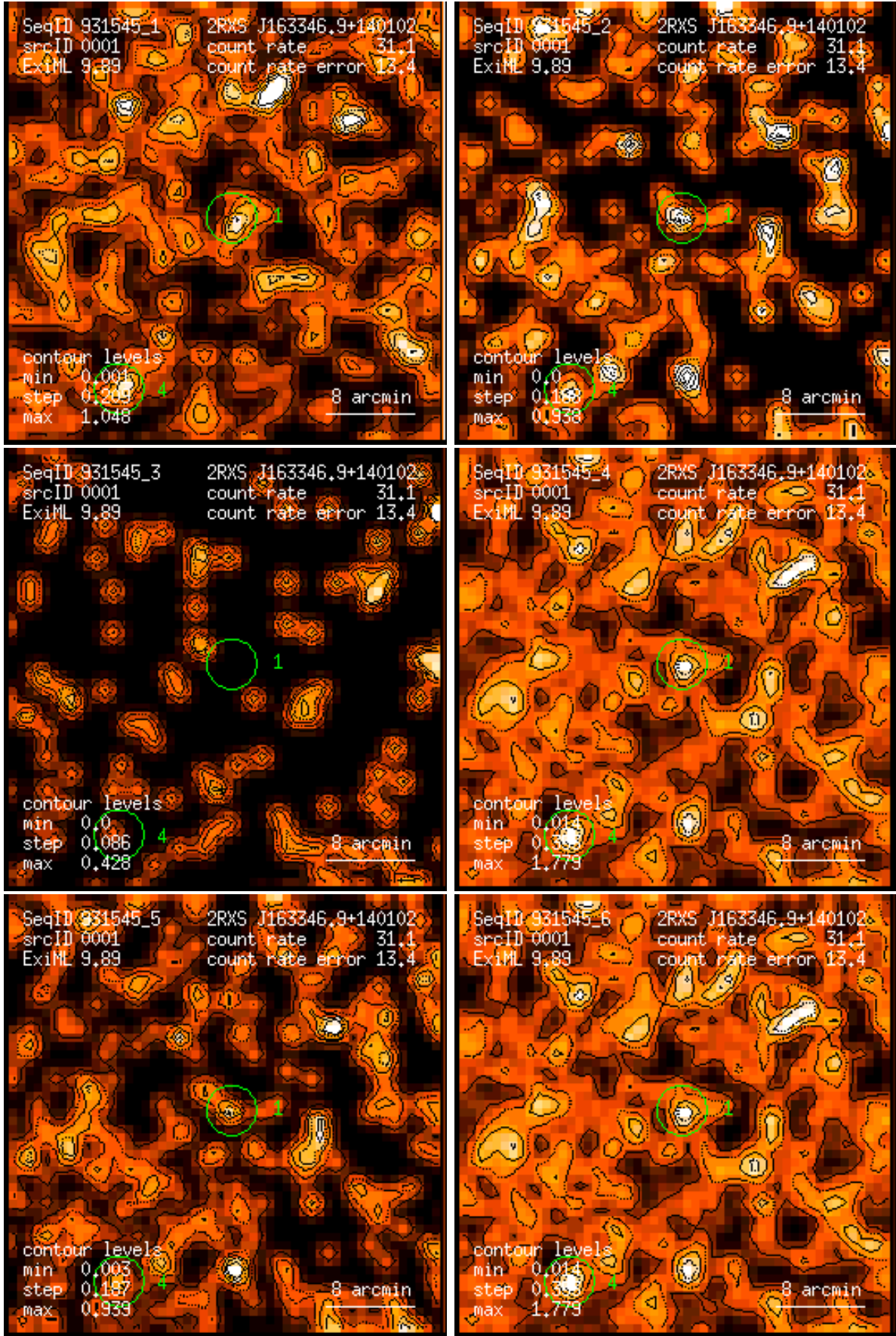
Figure 1: RASS 931545: detection 0001: band rate images, Gaussian filter: (1) PSPC channels 11 – 41, (2) 52 – 90, (3) 91 – 201, (4) 11 – 235, (5) 52 – 201, (6) 11 – 201. Broad band rates in counts/ks. Band rate contour levels in counts/ks/arcmin 2 .
