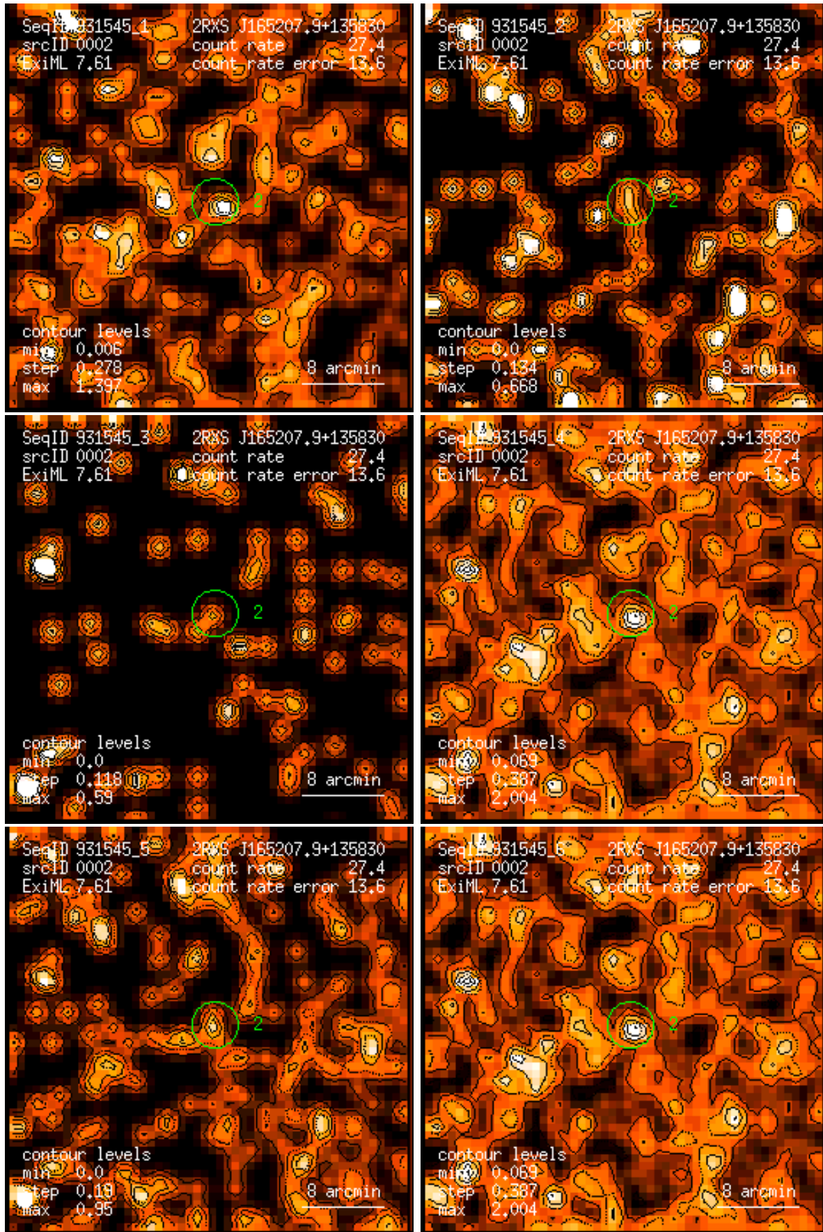
Figure 2: RASS 931545: detection 0002: band rate images, Gaussian filter: (1) PSPC channels 11 – 41, (2) 52 – 90, (3) 91 – 201, (4) 11 – 235, (5) 52 – 201, (6) 11 – 201. Broad band rates in counts/ks. Band rate contour levels in counts/ks/arcmin 2 .
