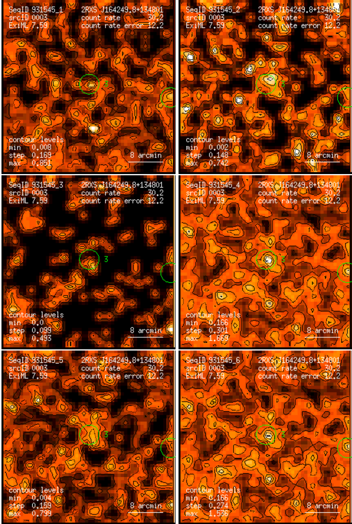
Figure 3: RASS 931545: detection 0003: band rate images, Gaussian filter: (1) PSPC channels 11 – 41, (2) 52 – 90, (3) 91 – 201, (4) 11 – 235, (5) 52 – 201, (6) 11 – 201. Broad band rates in counts/ks. Band rate contour levels in counts/ks/arcmin 2 .
