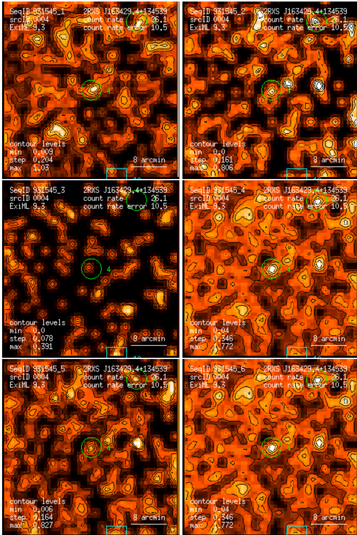
Figure 4: RASS 931545: detection 0004: band rate images, Gaussian filter: (1) PSPC channels 11 – 41, (2) 52 – 90, (3) 91 – 201, (4) 11 – 235, (5) 52 – 201, (6) 11 – 201. Broad band rates in counts/ks. Band rate contour levels in counts/ks/arcmin 2 .
