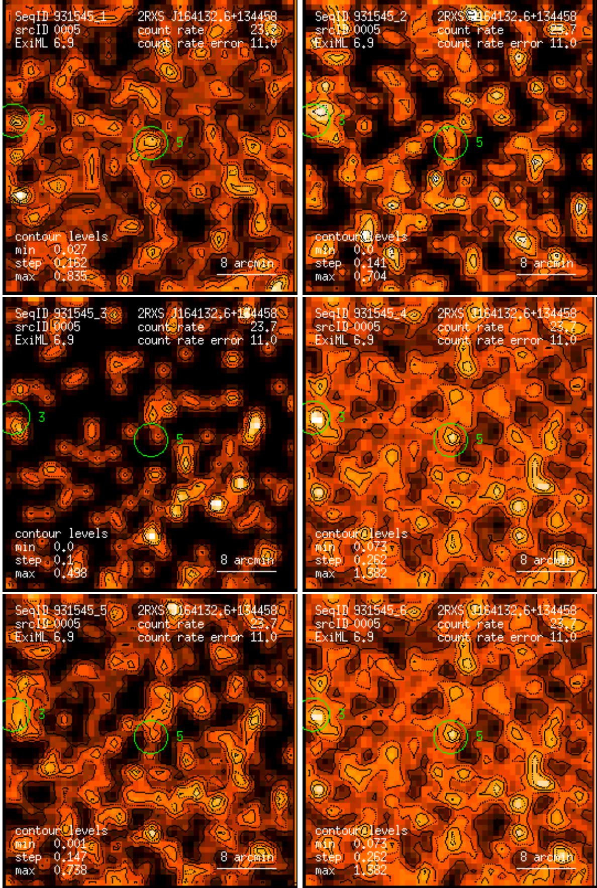
Figure 5: RASS 931545: detection 0005: band rate images, Gaussian filter: (1) PSPC channels 11 – 41, (2) 52 – 90, (3) 91 – 201, (4) 11 – 235, (5) 52 – 201, (6) 11 – 201. Broad band rates in counts/ks. Band rate contour levels in counts/ks/arcmin 2 .
