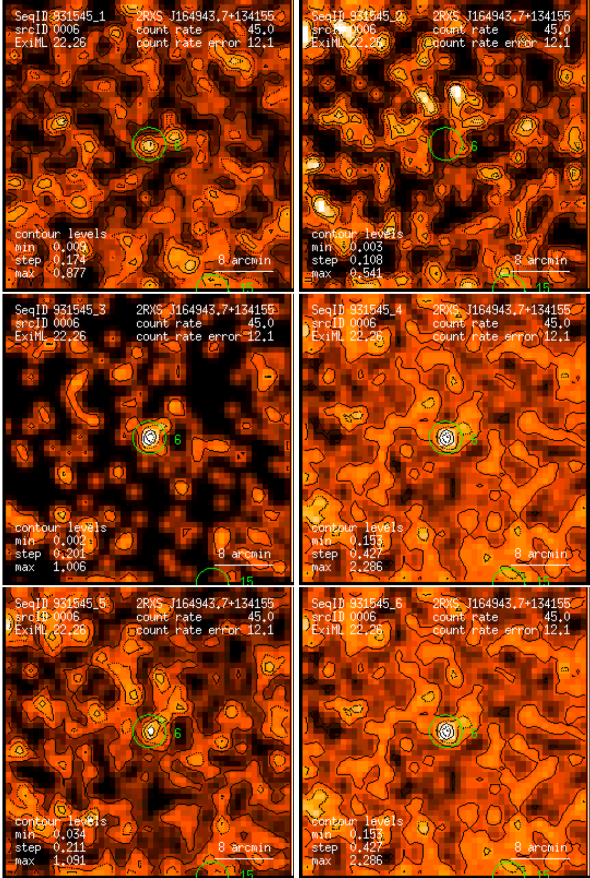
Figure 6: RASS 931545: detection 0006: band rate images, Gaussian filter: (1) PSPC channels 11 – 41, (2) 52 – 90, (3) 91 – 201, (4) 11 – 235, (5) 52 – 201, (6) 11 – 201. Broad band rates in counts/ks. Band rate contour levels in counts/ks/arcmin 2 .
