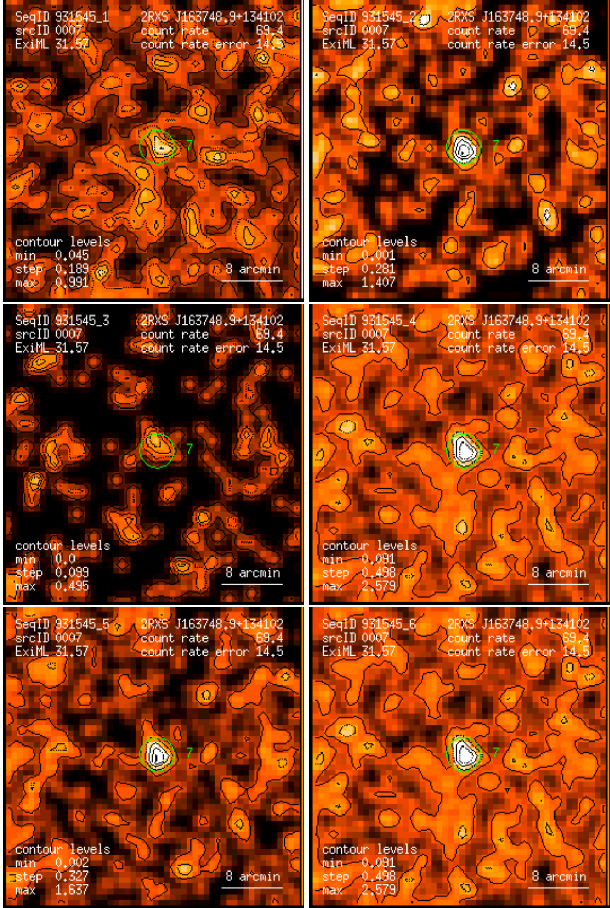
Figure 7: RASS 931545: detection 0007: band rate images, Gaussian filter: (1) PSPC channels 11 – 41, (2) 52 – 90, (3) 91 – 201, (4) 11 – 235, (5) 52 – 201, (6) 11 – 201. Broad band rates in counts/ks. Band rate contour levels in counts/ks/arcmin 2 .
