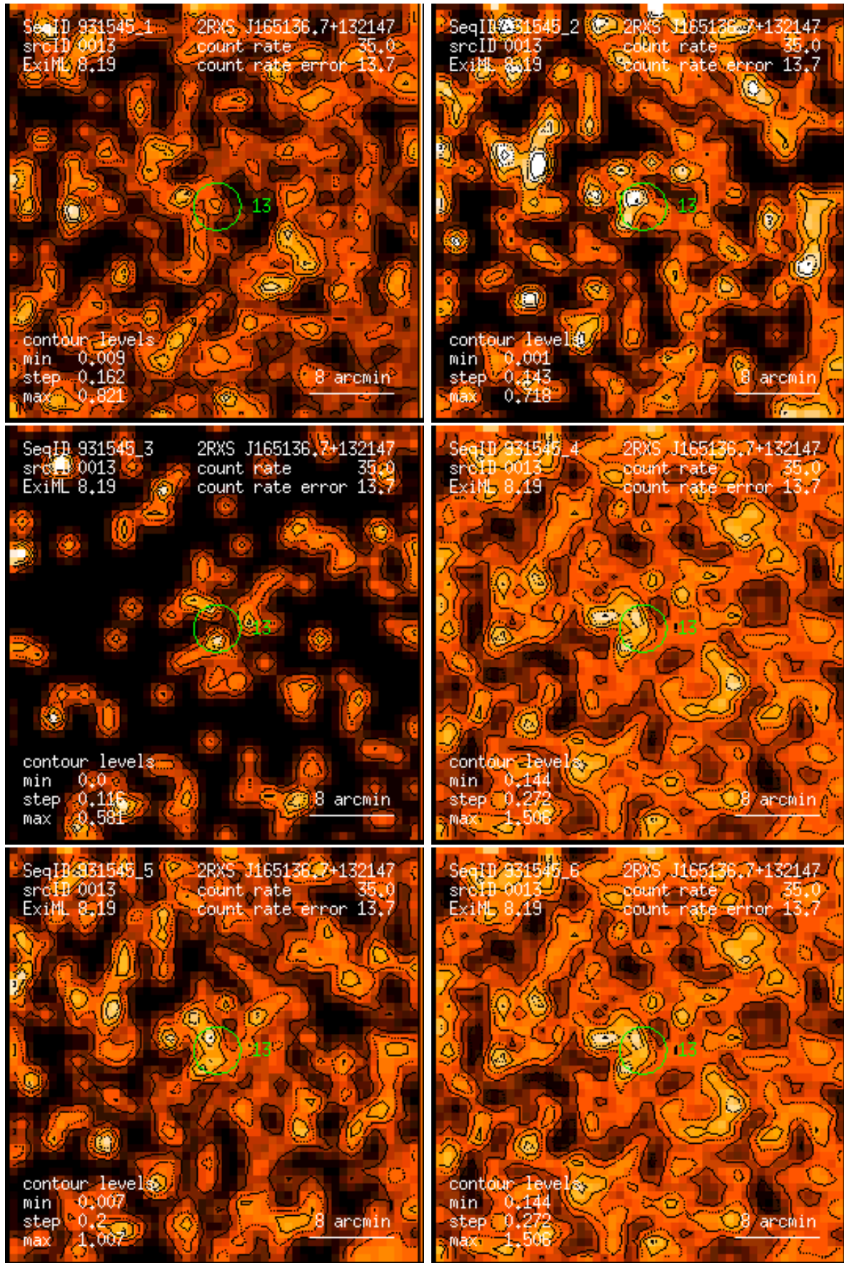
Figure 13: RASS 931545: detection 0013: band rate images, Gaussian filter: (1) PSPC channels 11 – 41, (2) 52 – 90, (3) 91 – 201, (4) 11 – 235, (5) 52 – 201, (6) 11 – 201. Broad band rates in counts/ks. Band rate contour levels in counts/ks/arcmin 2 .
