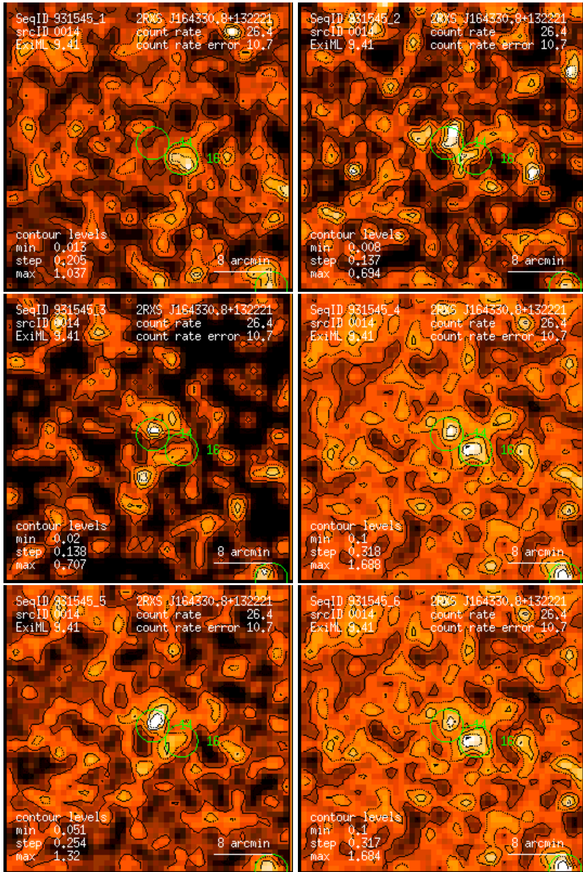
Figure 14: RASS 931545: detection 0014: band rate images, Gaussian filter: (1) PSPC channels 11 – 41, (2) 52 – 90, (3) 91 – 201, (4) 11 – 235, (5) 52 – 201, (6) 11 – 201. Broad band rates in counts/ks. Band rate contour levels in counts/ks/arcmin 2 .
