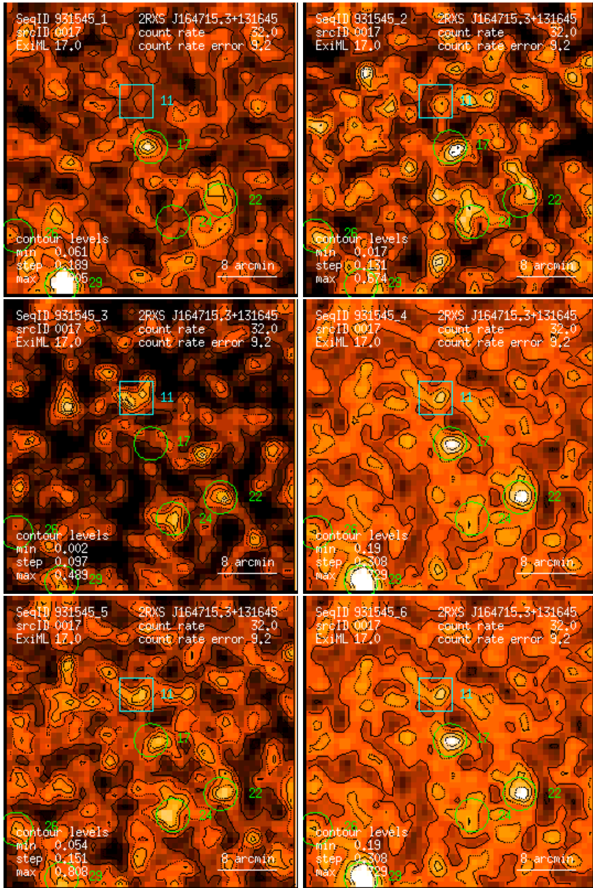
Figure 17: RASS 931545: detection 0017: band rate images, Gaussian filter: (1) PSPC channels 11 – 41, (2) 52 – 90, (3) 91 – 201, (4) 11 – 235, (5) 52 – 201, (6) 11 – 201. Broad band rates in counts/ks. Band rate contour levels in counts/ks/arcmin 2 .
