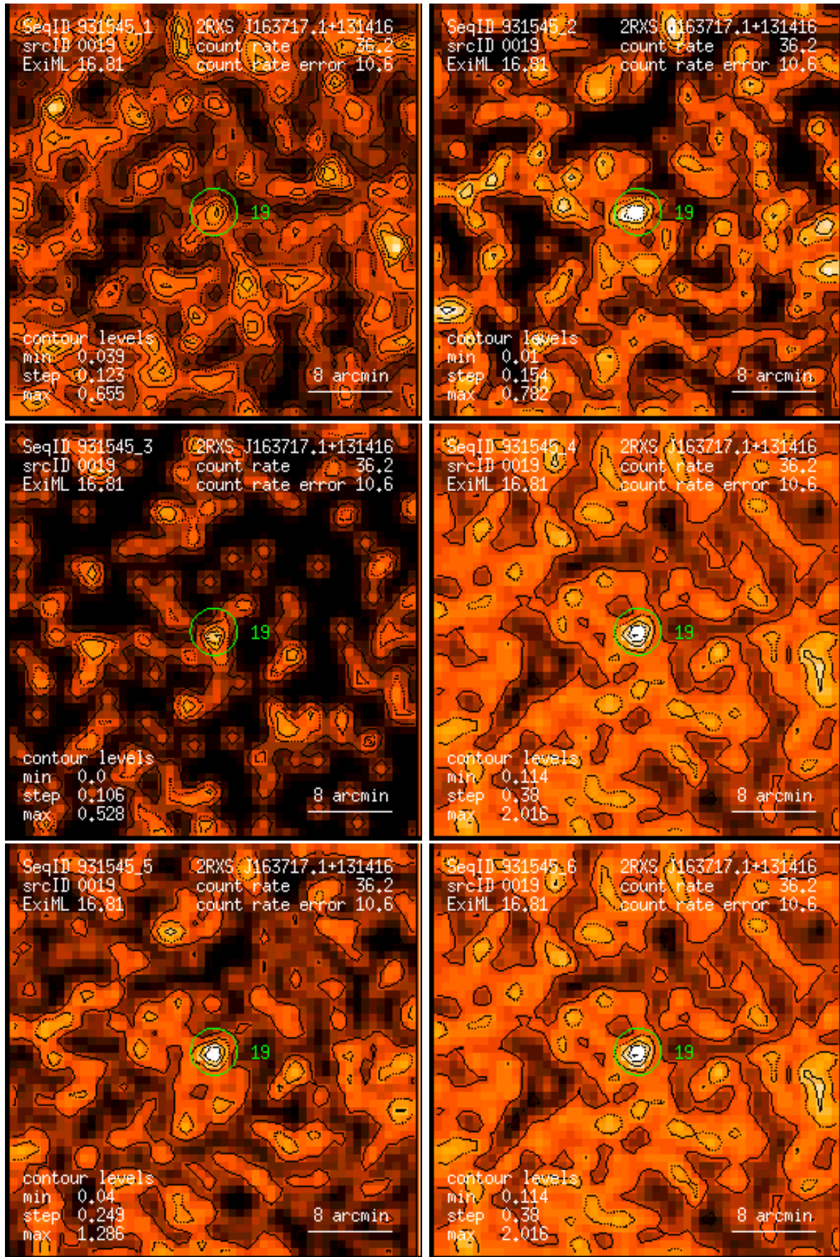
Figure 19: RASS 931545: detection 0019: band rate images, Gaussian filter: (1) PSPC channels 11 – 41, (2) 52 – 90, (3) 91 – 201, (4) 11 – 235, (5) 52 – 201, (6) 11 – 201. Broad band rates in counts/ks. Band rate contour levels in counts/ks/arcmin 2 .
