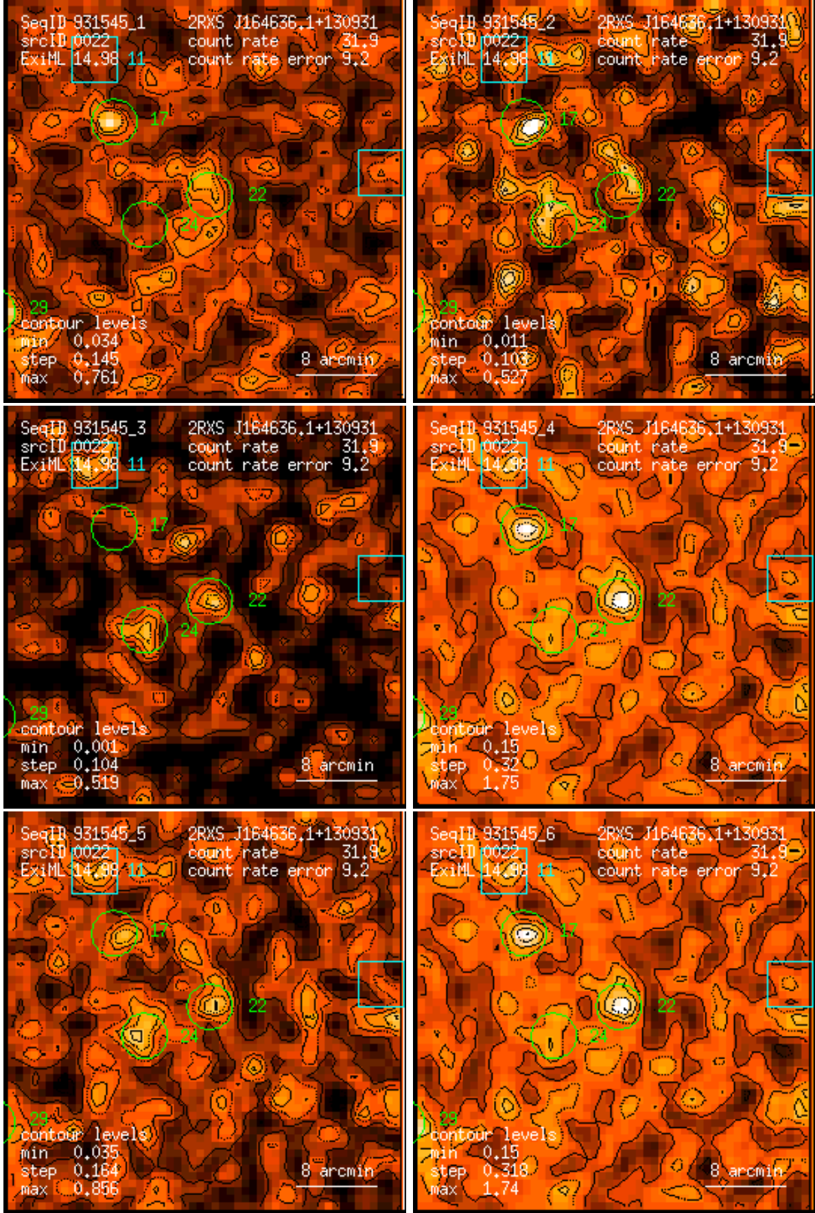
Figure 22: RASS 931545: detection 0022: band rate images, Gaussian filter: (1) PSPC channels 11 – 41, (2) 52 – 90, (3) 91 – 201, (4) 11 – 235, (5) 52 – 201, (6) 11 – 201. Broad band rates in counts/ks. Band rate contour levels in counts/ks/arcmin 2 .
