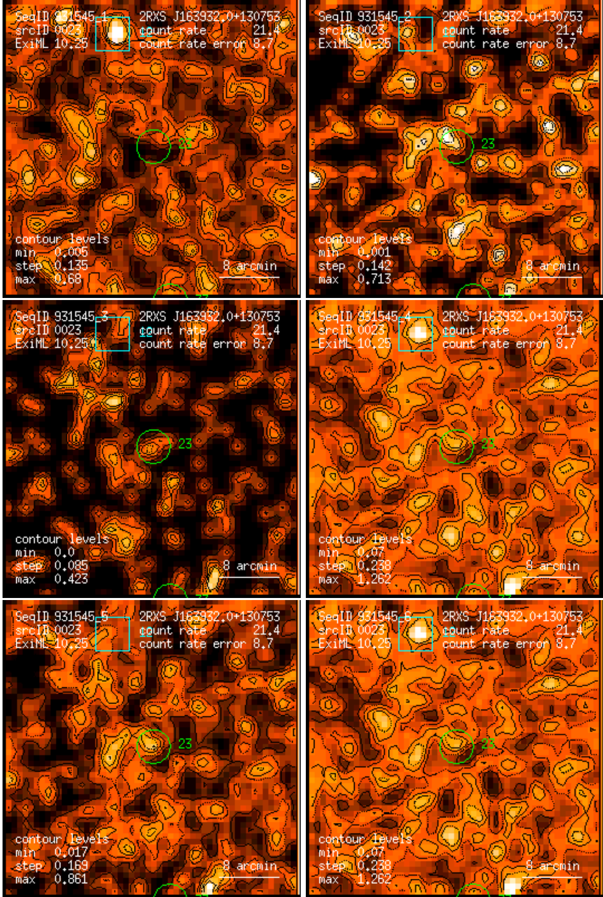
Figure 23: RASS 931545: detection 0023: band rate images, Gaussian filter: (1) PSPC channels 11 – 41, (2) 52 – 90, (3) 91 – 201, (4) 11 – 235, (5) 52 – 201, (6) 11 – 201. Broad band rates in counts/ks. Band rate contour levels in counts/ks/arcmin 2 .
