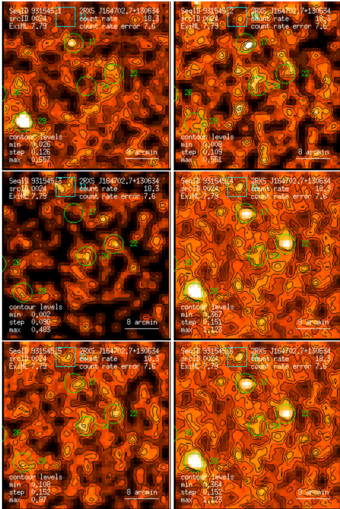
Figure 24: RASS 931545: detection 0024: band rate images, Gaussian filter: (1) PSPC channels 11 – 41, (2) 52 – 90, (3) 91 – 201, (4) 11 – 235, (5) 52 – 201, (6) 11 – 201. Broad band rates in counts/ks. Band rate contour levels in counts/ks/arcmin 2 .
