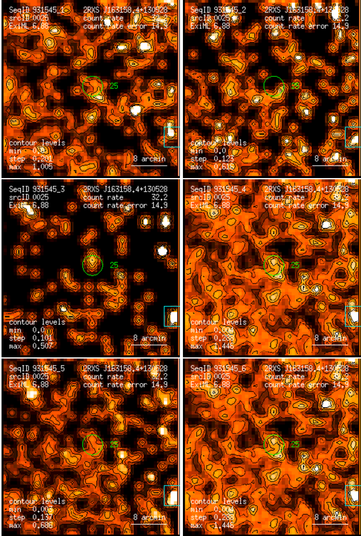
Figure 25: RASS 931545: detection 0025: band rate images, Gaussian filter: (1) PSPC channels 11 – 41, (2) 52 – 90, (3) 91 – 201, (4) 11 – 235, (5) 52 – 201, (6) 11 – 201. Broad band rates in counts/ks. Band rate contour levels in counts/ks/arcmin 2 .
