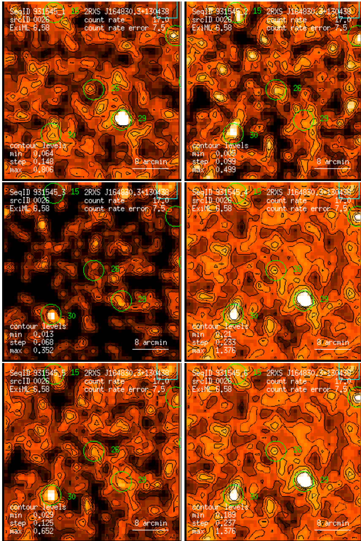
Figure 26: RASS 931545: detection 0026: band rate images, Gaussian filter: (1) PSPC channels 11 – 41, (2) 52 – 90, (3) 91 – 201, (4) 11 – 235, (5) 52 – 201, (6) 11 – 201. Broad band rates in counts/ks. Band rate contour levels in counts/ks/arcmin 2 .
