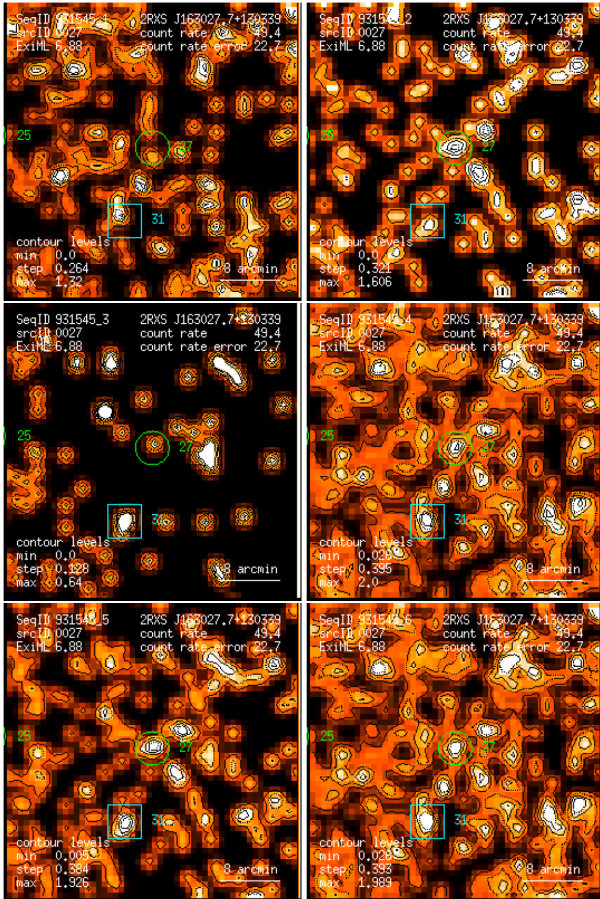
Figure 27: RASS 931545: detection 0027: band rate images, Gaussian filter: (1) PSPC channels 11 – 41, (2) 52 – 90, (3) 91 – 201, (4) 11 – 235, (5) 52 – 201, (6) 11 – 201. Broad band rates in counts/ks. Band rate contour levels in counts/ks/arcmin 2 .
