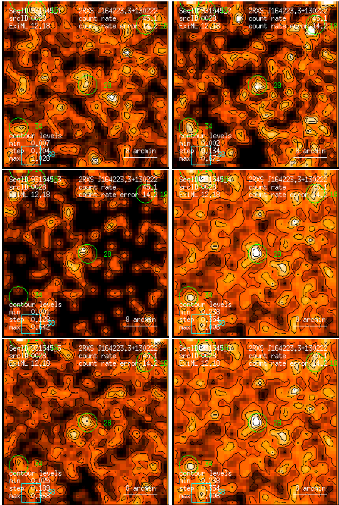
Figure 28: RASS 931545: detection 0028: band rate images, Gaussian filter: (1) PSPC channels 11 – 41, (2) 52 – 90, (3) 91 – 201, (4) 11 – 235, (5) 52 – 201, (6) 11 – 201. Broad band rates in counts/ks. Band rate contour levels in counts/ks/arcmin 2 .
