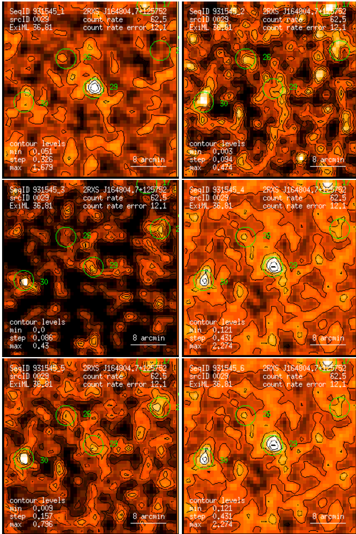
Figure 29: RASS 931545: detection 0029: band rate images, Gaussian filter: (1) PSPC channels 11 – 41, (2) 52 – 90, (3) 91 – 201, (4) 11 – 235, (5) 52 – 201, (6) 11 – 201. Broad band rates in counts/ks. Band rate contour levels in counts/ks/arcmin 2 .
