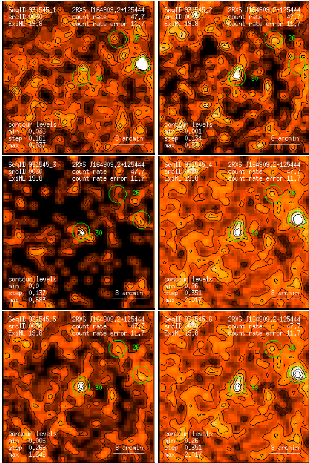
Figure 30: RASS 931545: detection 0030: band rate images, Gaussian filter: (1) PSPC channels 11 – 41, (2) 52 – 90, (3) 91 – 201, (4) 11 – 235, (5) 52 – 201, (6) 11 – 201. Broad band rates in counts/ks. Band rate contour levels in counts/ks/arcmin 2 .
