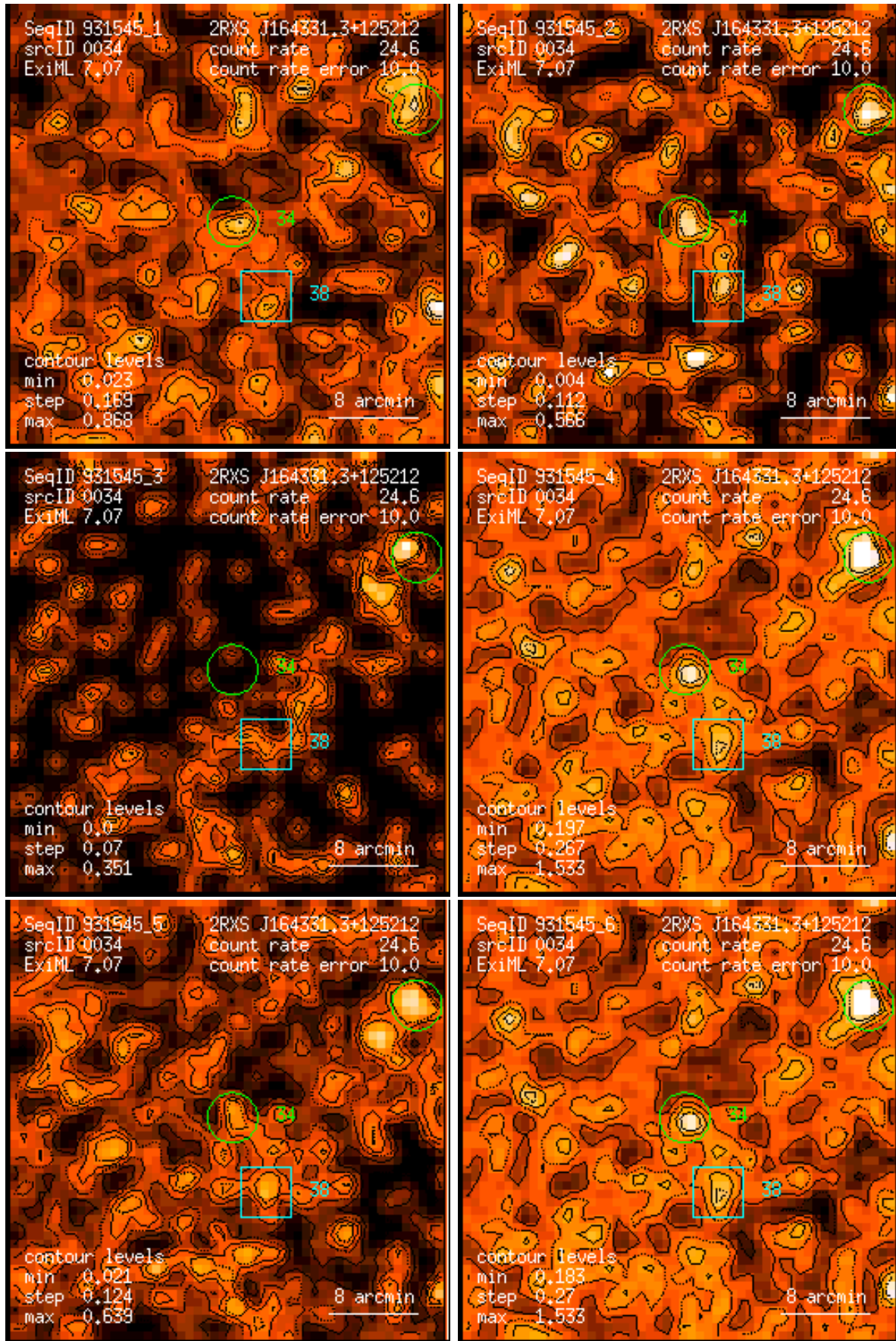
Figure 34: RASS 931545: detection 0034: band rate images, Gaussian filter: (1) PSPC channels 11 – 41, (2) 52 – 90, (3) 91 – 201, (4) 11 – 235, (5) 52 – 201, (6) 11 – 201. Broad band rates in counts/ks. Band rate contour levels in counts/ks/arcmin 2 .
