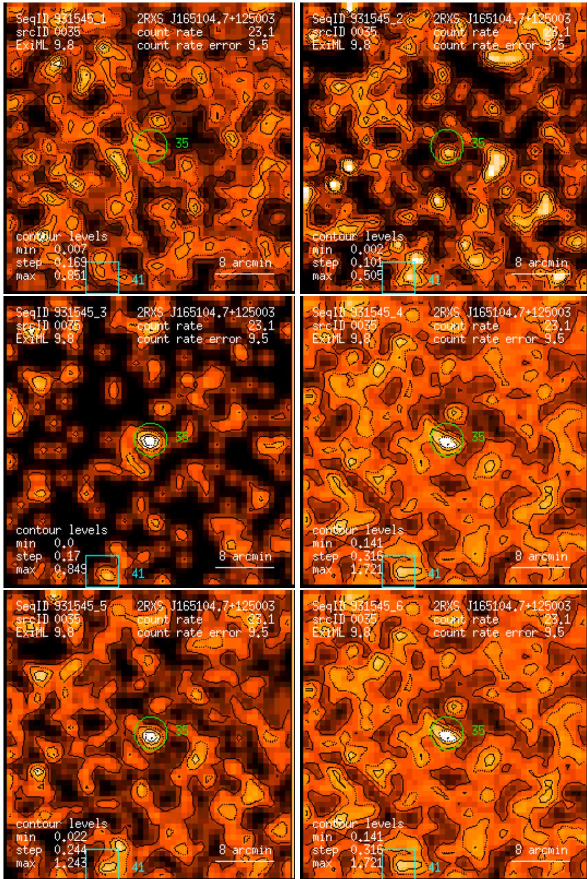
Figure 35: RASS 931545: detection 0035: band rate images, Gaussian filter: (1) PSPC channels 11 – 41, (2) 52 – 90, (3) 91 – 201, (4) 11 – 235, (5) 52 – 201, (6) 11 – 201. Broad band rates in counts/ks. Band rate contour levels in counts/ks/arcmin 2 .
