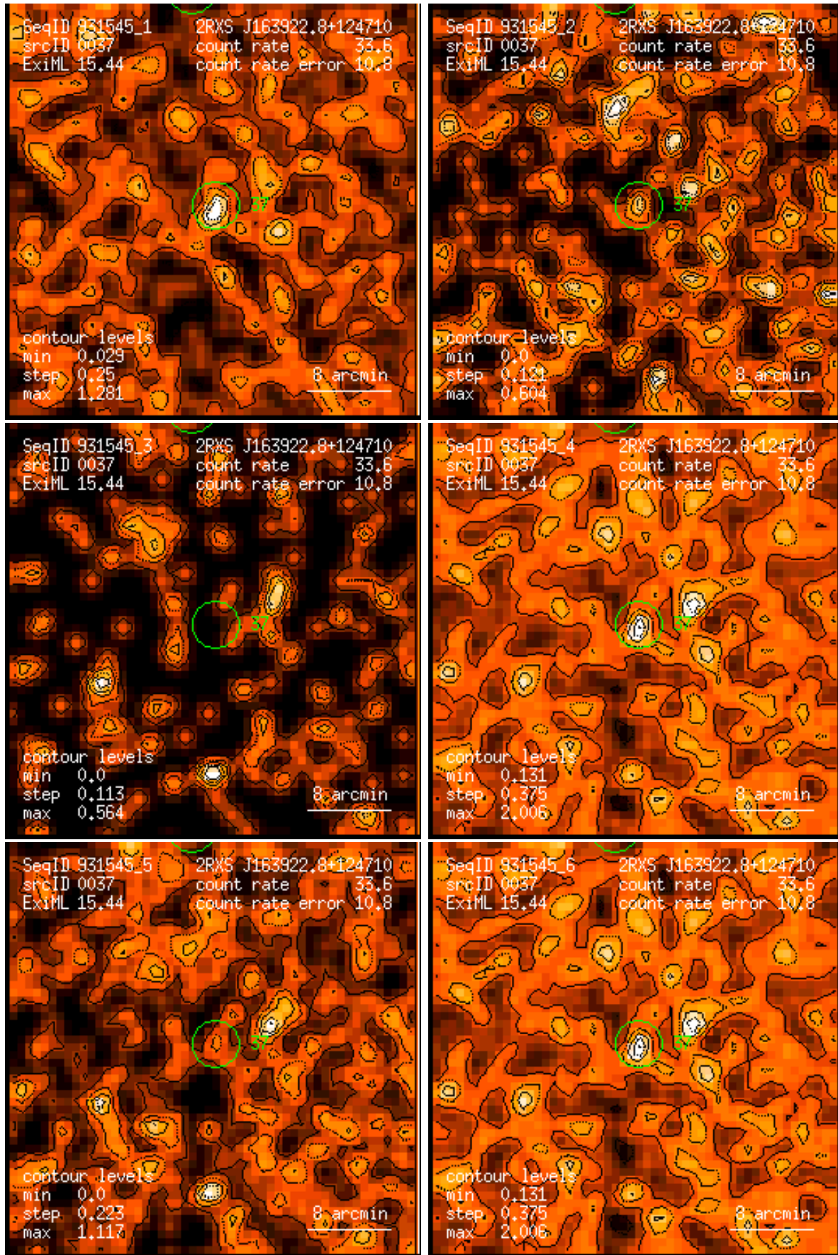
Figure 37: RASS 931545: detection 0037: band rate images, Gaussian filter: (1) PSPC channels 11 – 41, (2) 52 – 90, (3) 91 – 201, (4) 11 – 235, (5) 52 – 201, (6) 11 – 201. Broad band rates in counts/ks. Band rate contour levels in counts/ks/arcmin 2 .
