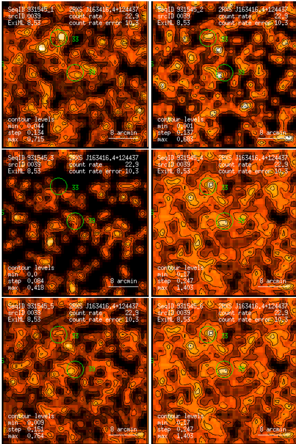
Figure 39: RASS 931545: detection 0039: band rate images, Gaussian filter: (1) PSPC channels 11 – 41, (2) 52 – 90, (3) 91 – 201, (4) 11 – 235, (5) 52 – 201, (6) 11 – 201. Broad band rates in counts/ks. Band rate contour levels in counts/ks/arcmin 2 .
