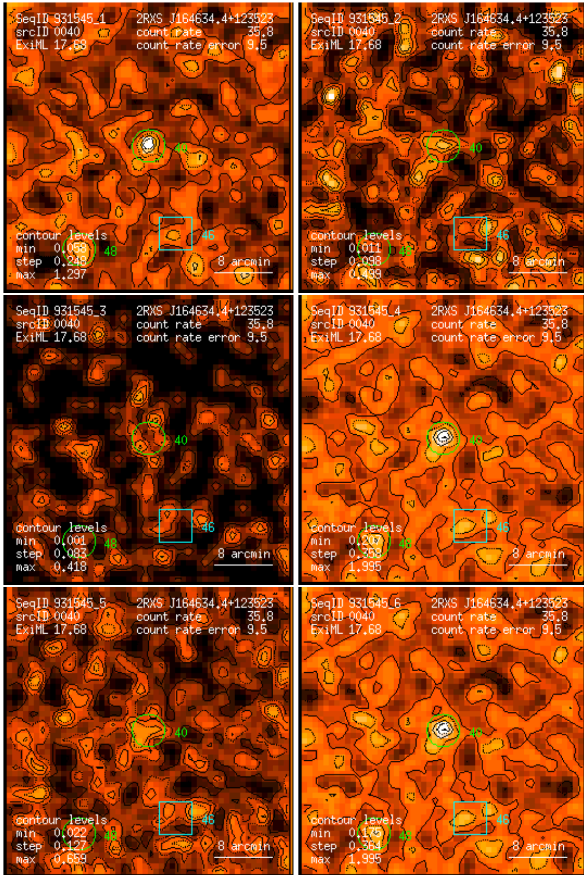
Figure 40: RASS 931545: detection 0040: band rate images, Gaussian filter: (1) PSPC channels 11 – 41, (2) 52 – 90, (3) 91 – 201, (4) 11 – 235, (5) 52 – 201, (6) 11 – 201. Broad band rates in counts/ks. Band rate contour levels in counts/ks/arcmin 2 .
