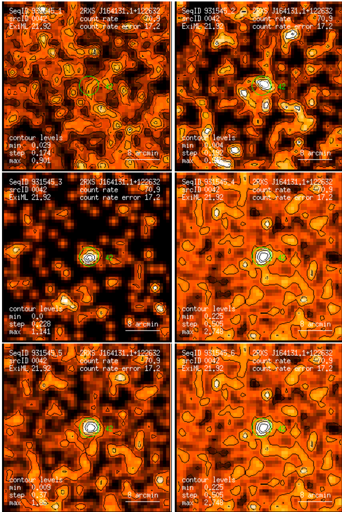
Figure 42: RASS 931545: detection 0042: band rate images, Gaussian filter: (1) PSPC channels 11 – 41, (2) 52 – 90, (3) 91 – 201, (4) 11 – 235, (5) 52 – 201, (6) 11 – 201. Broad band rates in counts/ks. Band rate contour levels in counts/ks/arcmin 2 .
